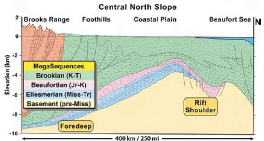
Figure 4.10. North Slope stratigraphy. (Courtesy of Dave Houseknecht, U.S. Geological Survey)
