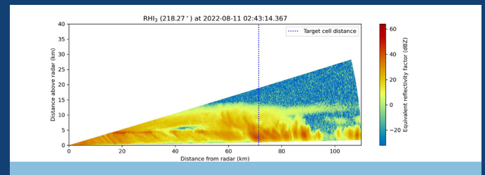
This Py-ART image from ARM's TRACER campaign near Houston, Texas, showcases vertical cross-sections through deep convective cells.
