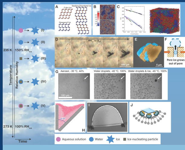
At the coldest temperatures, ice nucleates from aqueous solution (I) or water (II) droplets. Ice deposits from the supersaturated vapor phase onto an ice-nucleating particle (III). An ice-nucleating particle immersed in supercooled water (IV) or aqueous solution (V) can initiate freezing. (Copyrighted image from the journal.)
