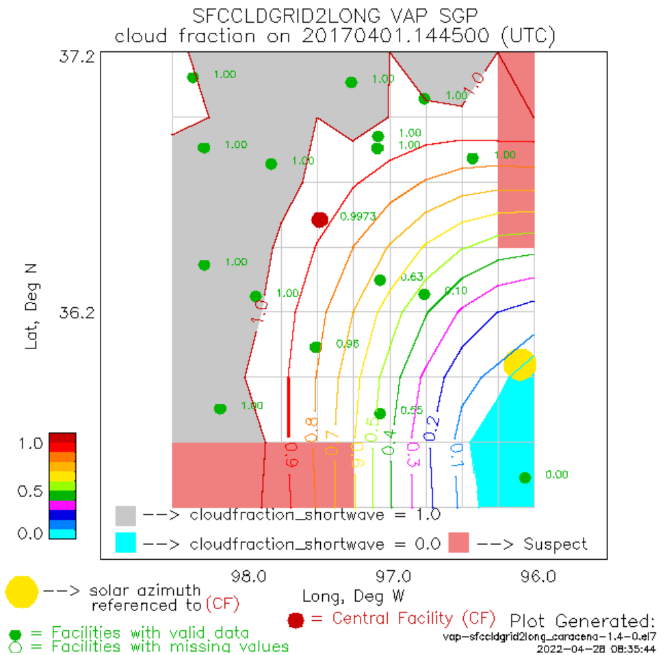
The figure illustrates SFCCLDGRID cloud fraction on the morning of April 1, 2017, when the Southern Great Plains (SGP) atmospheric observatory experienced partly cloudy conditions with clear skies to the east and overcast conditions to the west and north. The yellow ball represents the sun in the sky, the SGP Central Facility is noted in red, and other SGP facilities are noted in green.
