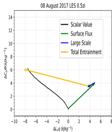
This mixing diagram shows the evolution of the convective boundary layer (black line), with the contributions from the surface (green), horizontal advection (blue), and entrainment from above (yellow). (Copyrighted image from the journal.)
