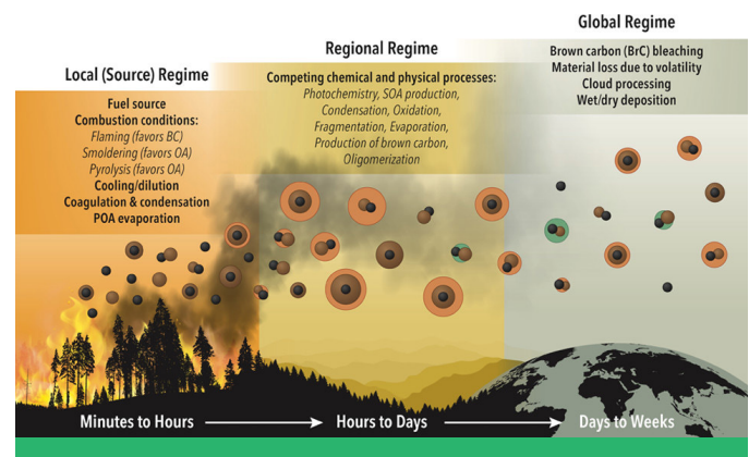
There are three primary regimes of wildfire particles. As the particles age, the processes that control their properties change, and the properties evolve. (Copyrighted image from the journal.)
