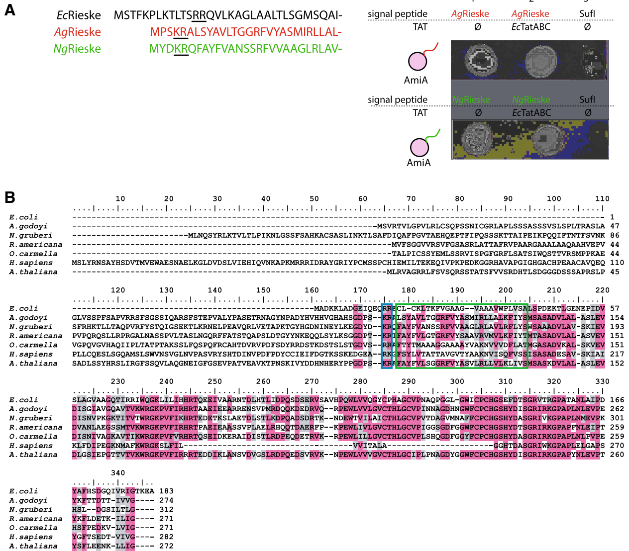
Fig. 4 Rieske proteins as putative substrate of mitochondrial TAT. a The experimental signal peptides of A. godoyi and N. gruberi Rieske proteins. Ag / Ng Rieske signal sequences fused to mature AmiA expressed from pSU18 are translocated through bacterial membrane in both absence (1; pTH19kr) and presence (2; pTAT101) of TAT in MCDSSAC \Delta tat strain. (3) SufI signal sequence fused to mature AmiA expressed from pSU18 is not translocated in the absence of TAT (pTH19kr) in MCDSSAC \Delta tat strain. b Protein sequence alignment of the Rieske protein orthologues shows the presence of putative twin arginine motif in both TAT-positive (TatAC in A. godoyi and R. americana , TatBC in A. thaliana , TatC-only in N. gruberi and O. carmella ) and TAT-negative eukaryotes ( H. sapiens ). The blue rectangle highlights the presence of twin arginine (RR) or derived (KR and RK) motifs, and the green rectangle depicts the transmembrane domain. Identical and similar residues are highlighted in pink and grey colour, respectively. The threshold for shading was 50%
