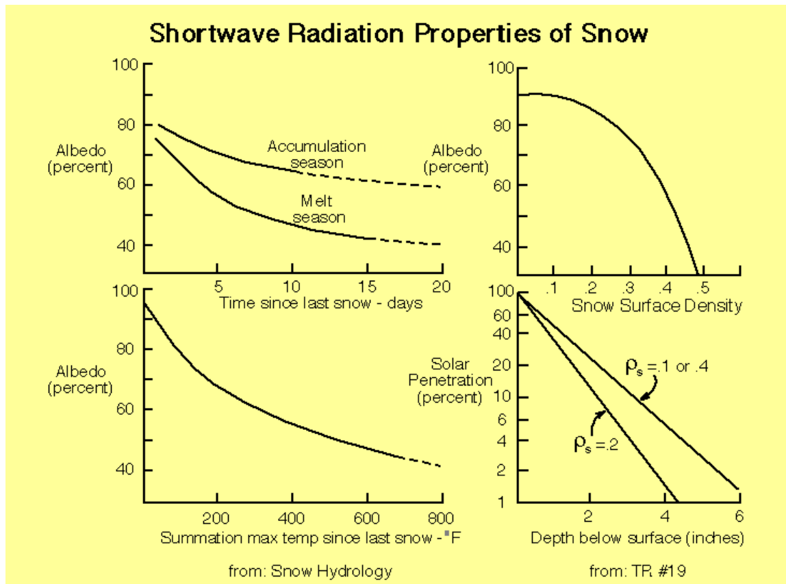
Figure A-4. Shortwave radiation properties of snow.
