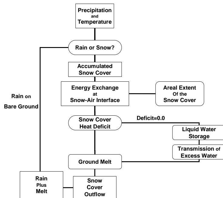
Figure 1. Flowchart of the SNOW-17 model
