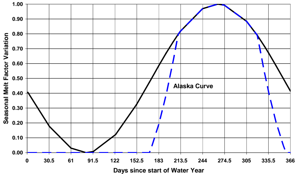
Figure 5. Seasonal melt factor variations used by SNOW-17.
