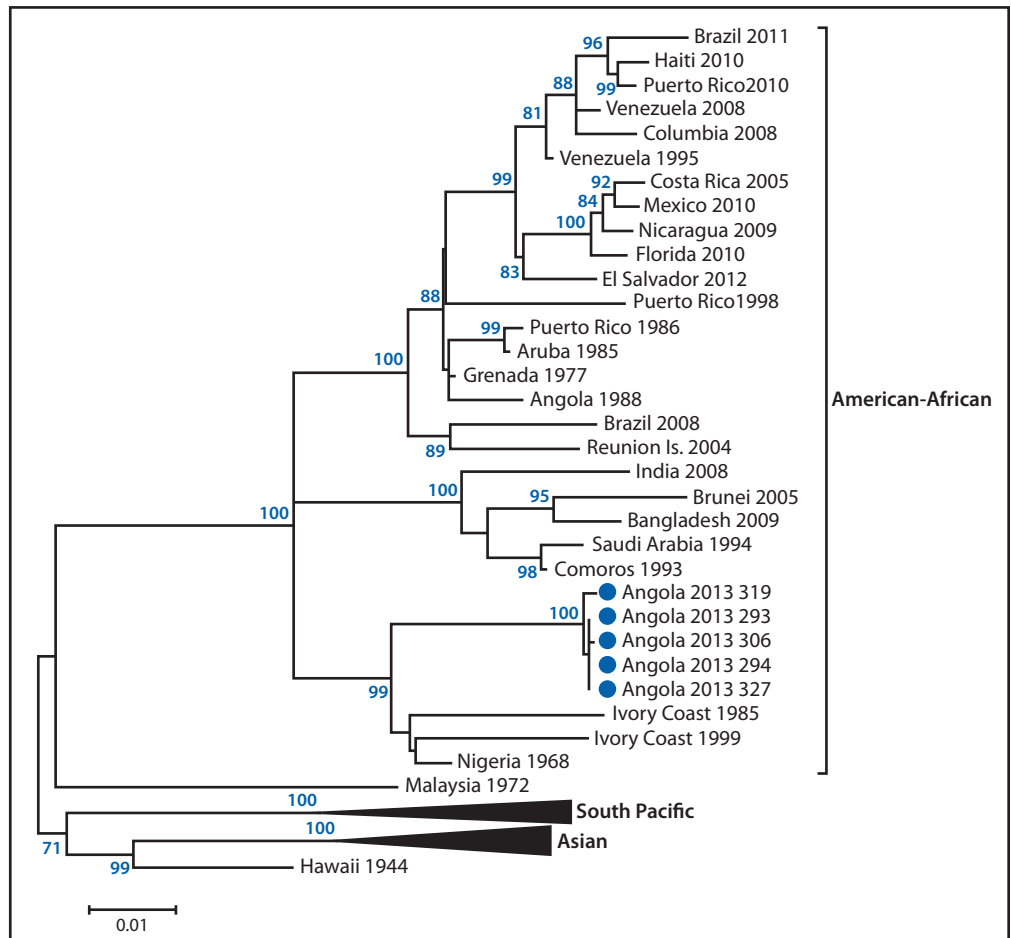
FIGURE 2. Phylogenetic tree* depicting the dengue virus-type 1 circulating in Angola in 2013
