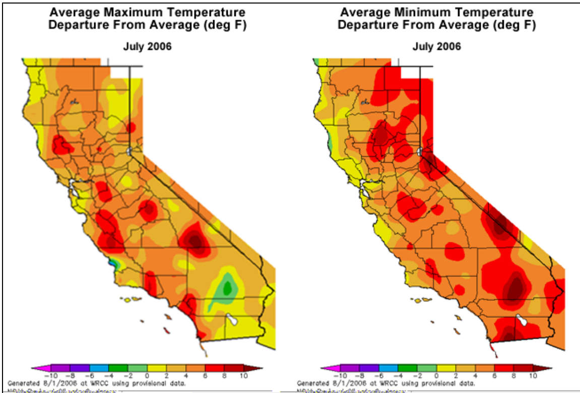
Figure 21: Depicts the departure from average for both the average maximum and average minimum temperature (°F) for July 2006. As one would expect, average maximum and average minimum temperature both exhibited above normal conditions across much of California. In fact, one of the aspects that made the July 2006 heat wave noteworthy was the elevated overnight minimum temperatures, which is reflected well in the right hand image.
