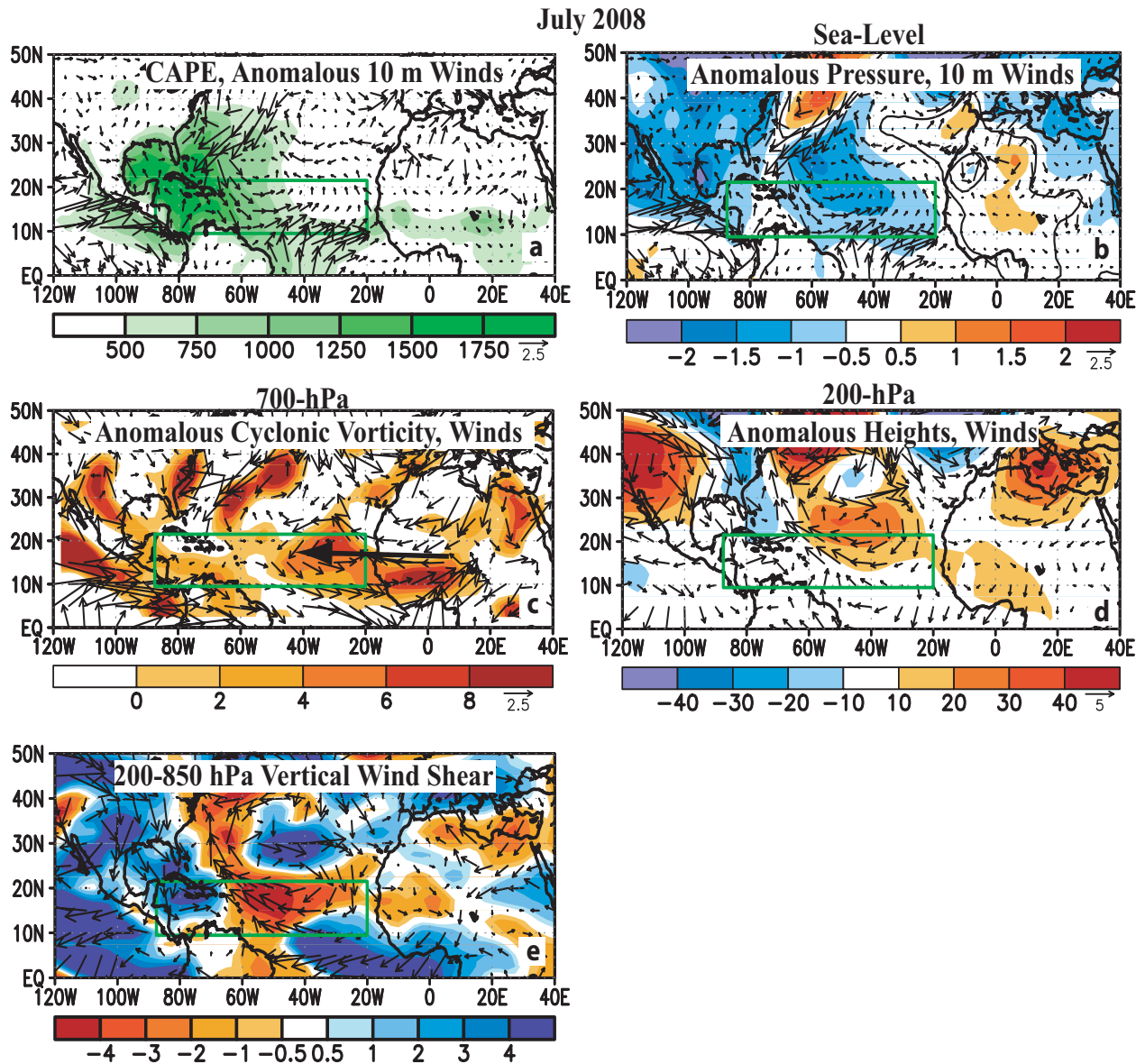
Fig. 12. July 2008: (a) Total CAPE ( \text{J kg}^{-1} ) and anomalous vector winds ( \text{m s}^{-1} ) at 10 m. (b) Anomalous sea-level pressure (shading, hPa) and vector winds at 10 m. (c) 700-hPa anomalous cyclonic relative vorticity (shading) and vector winds, with thick solid line indicating the observed AEJ core. (d) 200-hPa anomalous heights and vector winds. (e) 200-850 hPa vertical wind shear magnitude ( \text{m s}^{-1} ) and vectors. In (e), red (blue) shading indicates below- (above-) average magnitude of the vertical shear. Green boxes denote the MDR. Anomalies are departures from the 1971-2000 monthly means.
