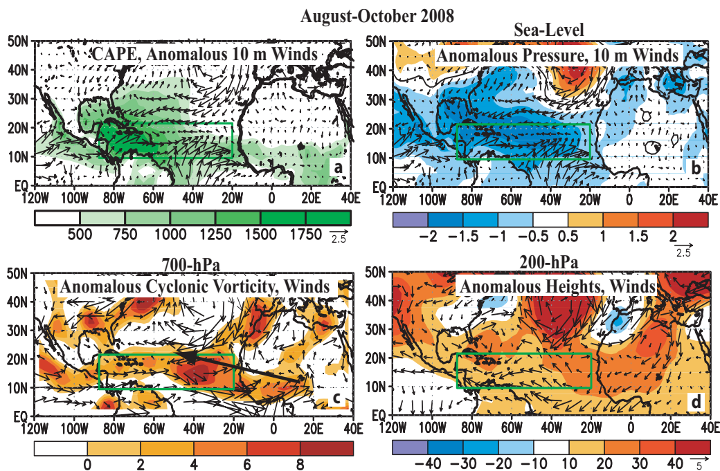
Fig. 5. Aug-Oct 2008: (a) Total CAPE ( \text{J kg}^{-1} ) and anomalous vector winds ( \text{m s}^{-1} ) at 10 m. (b) Anomalous sea-level pressure (shading, hPa) and vector winds at 10 m. (c) 700-hPa anomalous cyclonic relative vorticity (shading) and vector winds, with thick solid line indicating the observed AEJ core. (d) 200-hPa anomalous heights and vector winds. Green boxes denote the MDR. Anomalies are departures from the 1971-2000 monthly means.
