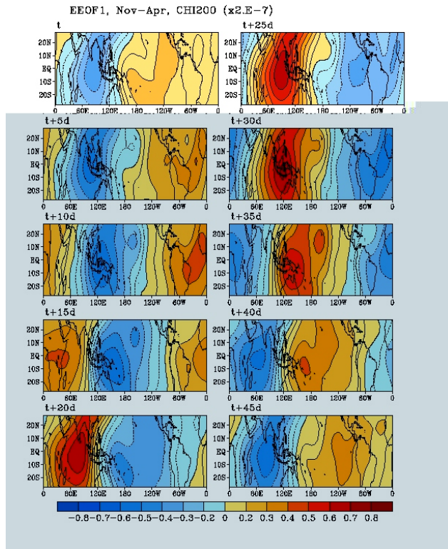
Fig. 1. The first EEOF of the pentad velocity potential at 200-hPa for the ENSO-neutral and weak ENSO winters (November-April) during 1979-2000.
