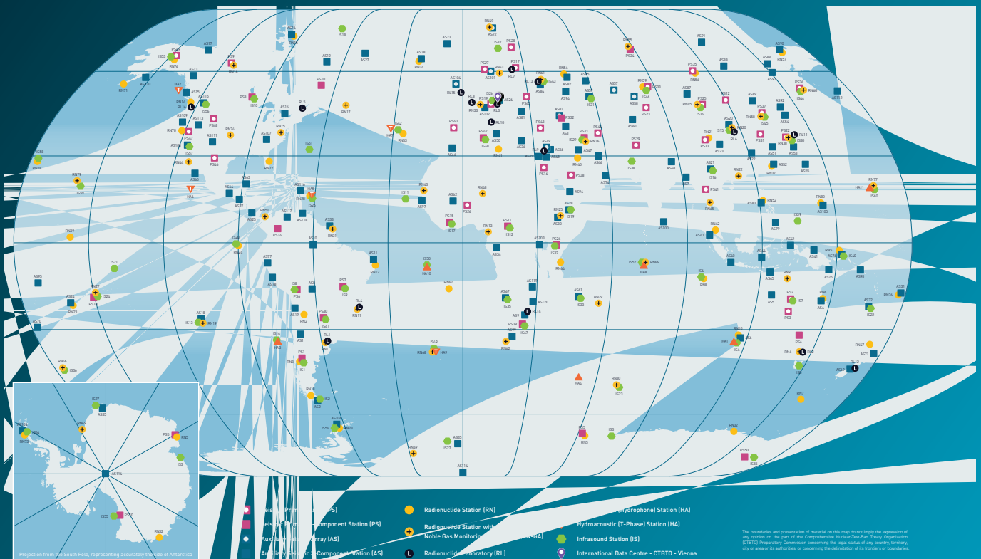
Over 300 stations using four technologies monitor planet Earth for nuclear explosions.
