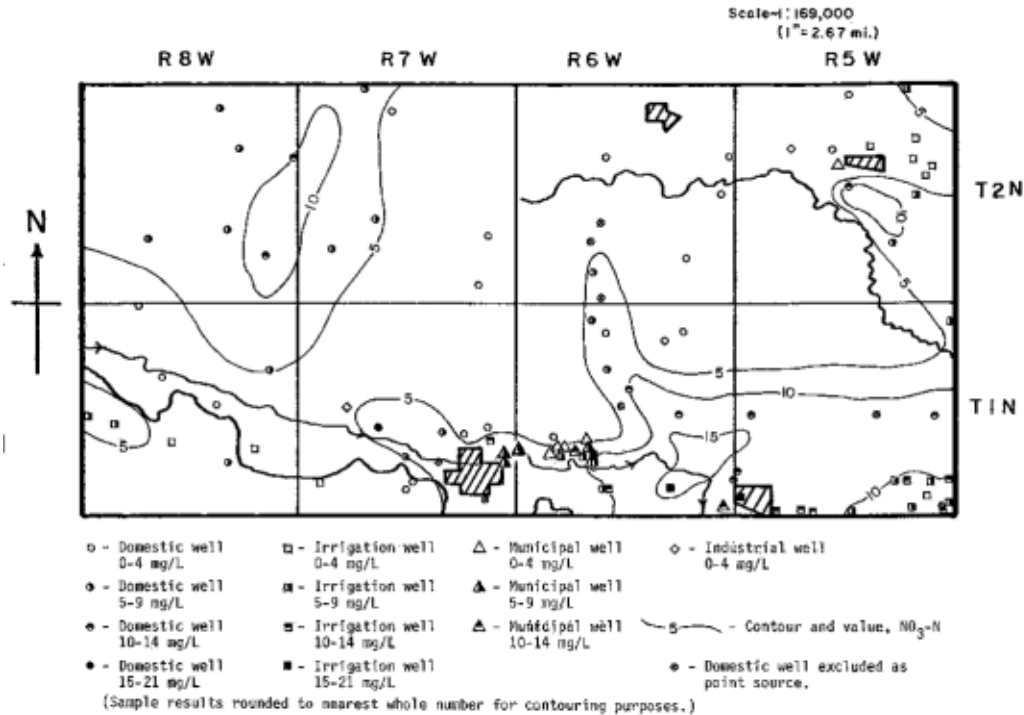
Figure 16: Sampling results and contour map of nitrate-nitrogen levels, study area
