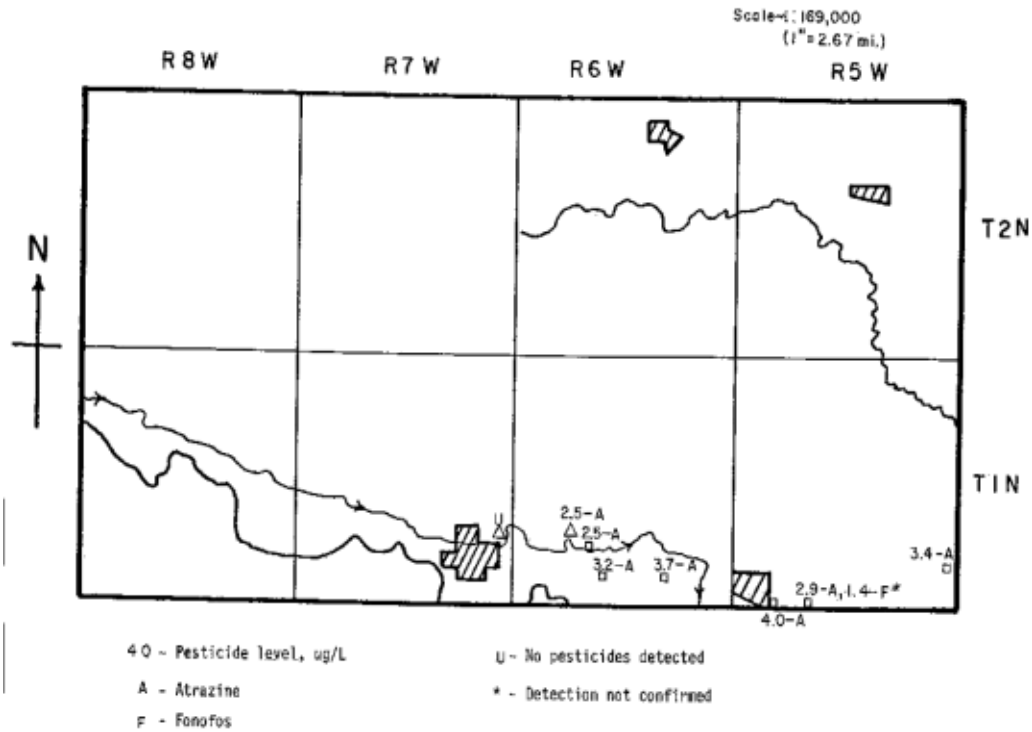
Figure 17: Locations and results of pesticide sampling
