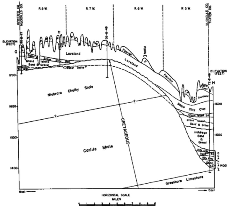
Figure 11: East -west cross-section through northern portion of study area (Reproduced with permission from CSD, 1948)
