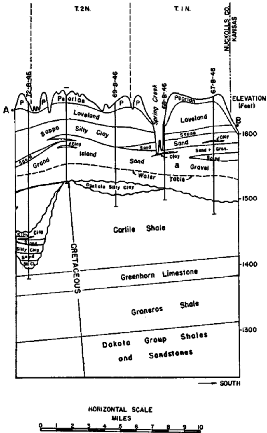
Figure 8: North-south cross-section along Nuckolls-Thayer County line (eastern border of study area) (Reproduced with permission from CSD, 1948)
