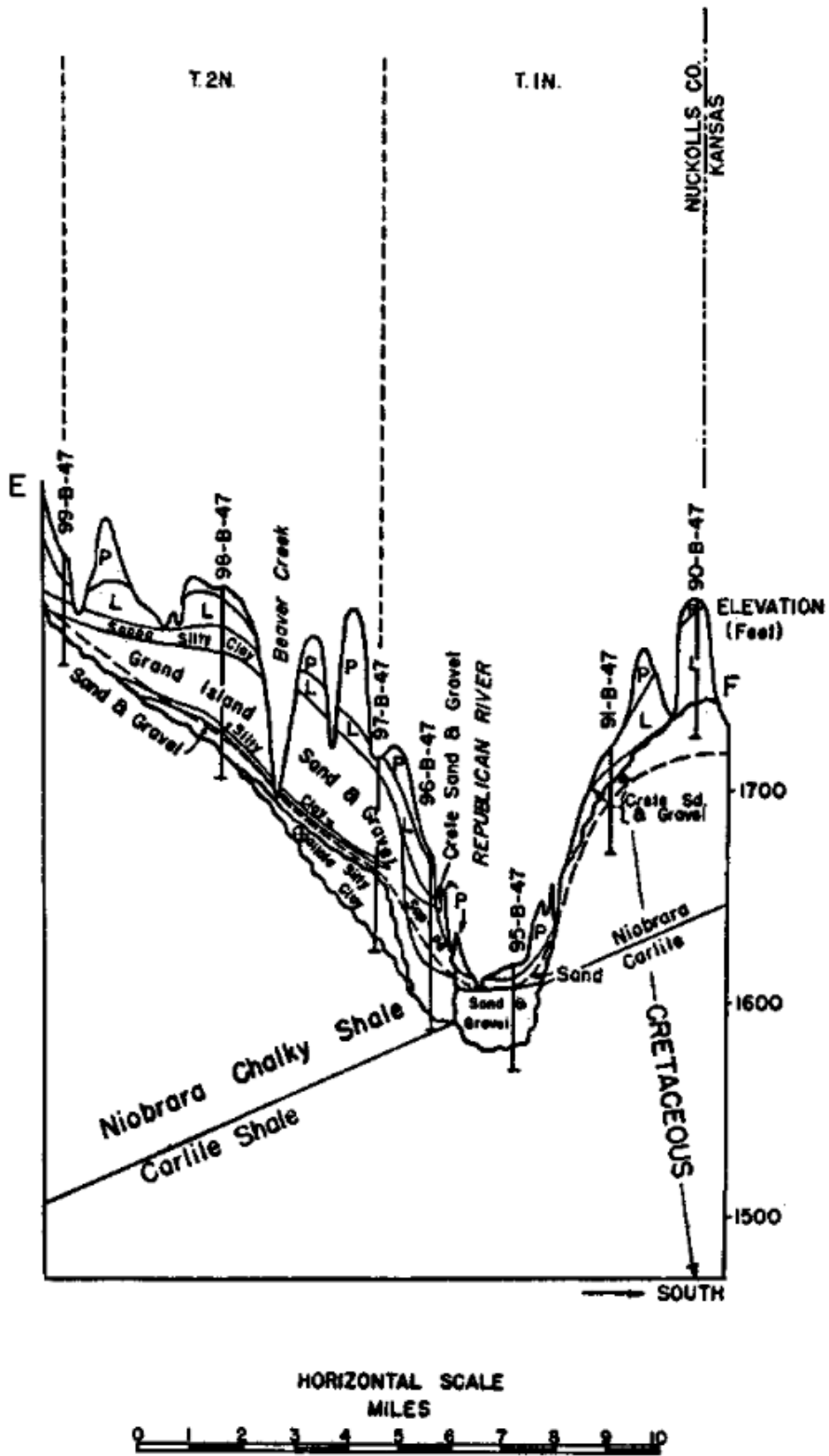
Figure 10: North-south cross-section along Nuckolls-Webster County line (western boundary of study area) (Reproduced with permission from CSD, 1948)
