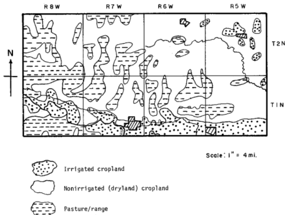
Figure 3: Generalized land use in the study area (Source: NRC Databank)
