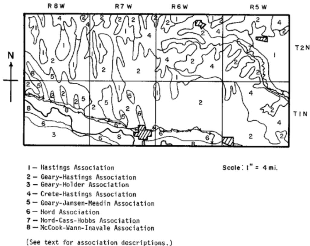
Figure 4: Generalized soil association map of study area (Redrawn from Pollock and Davis, 1978)
