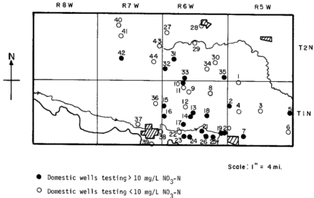
Figure 2: Locations and results of domestic well sampling submitted by LRNRD in request for SPA consideration
