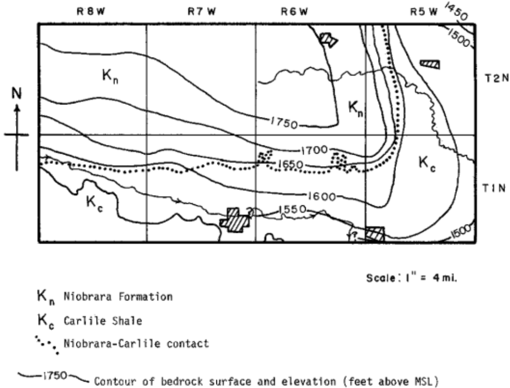
Figure 6: Contour map of upper bedrock surface, study area (Redrawn from Miller et al., 1964)
