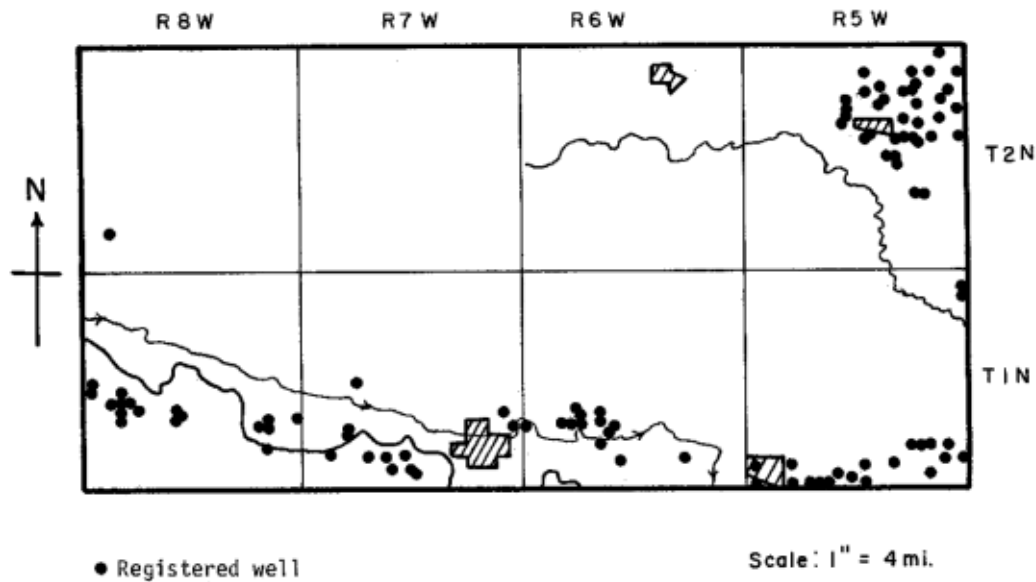
Figure 12: Location of registered wells in study area
