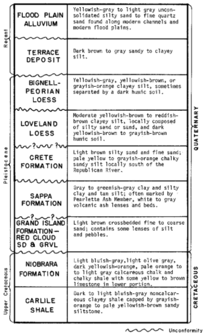
Figure 5: Stratigraphic section of units present in study area (Redrawn from Miller et al., 1964)
