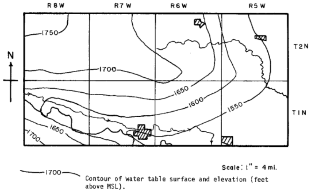
Figure 13: Generalized water table map of study area (Redrawn from DEC-CSD, 1980)
