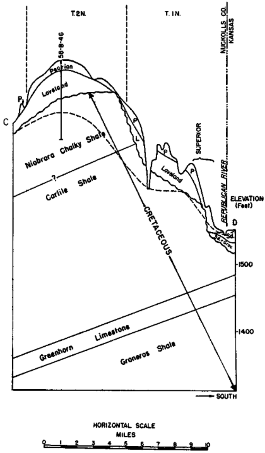
Figure 9: North-south cross-section through central portion of study area (Reproduced with permission from CSD, 1948)
