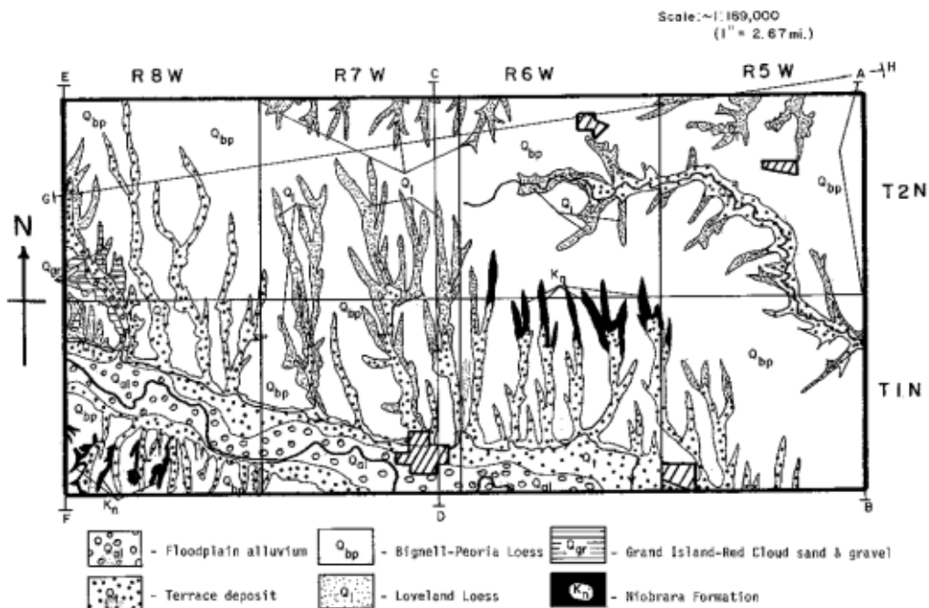
Figure 7: Generalized geologic map of study area, with location of cross-sections (Redrawn from Miller et al., 1964)
