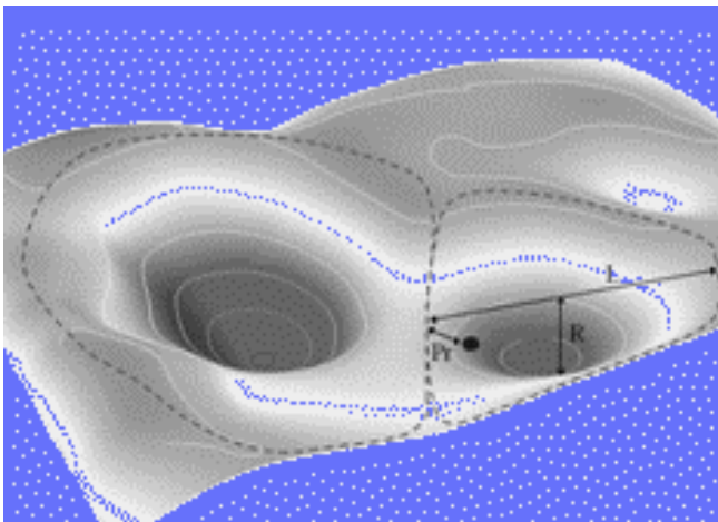
Fig. 1a. Three-dimensional stability landscape with two basins of attraction showing, in one basin, the current position of the system and three aspects of resilience, L = latitude, R = resistance, Pr = precariousness.
