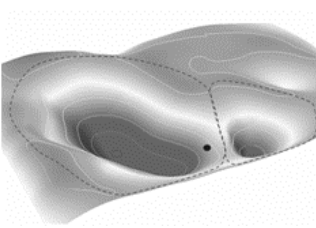
Fig. 1b. Changes in the stability landscape have resulted in a contraction of the basin the system was in and an expansion of the alternate basin. Without itself changing, the system has changed basins.
