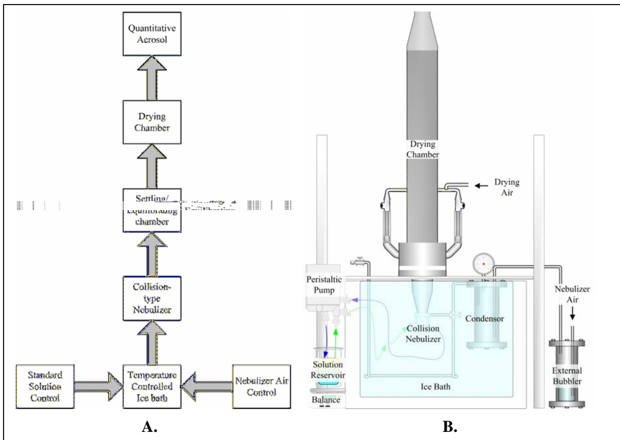
Figure 1: A. Schematic of flow through QAG components. B. Overview of the set-up of the CES QAG.
