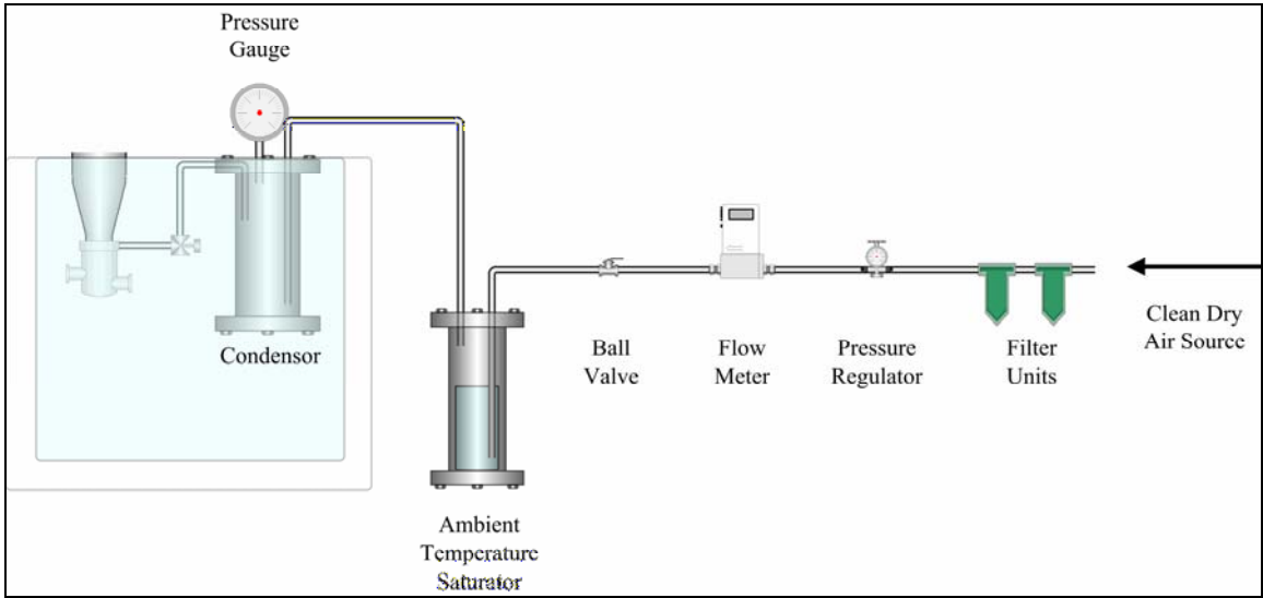
Figure 3: Schematic of the CES QAG nebulizer air control system.
