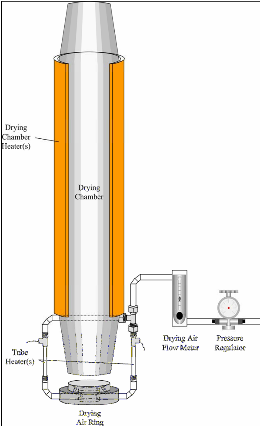
Figure 5: Schematic of the CES QAG drying air and drying chamber system.
