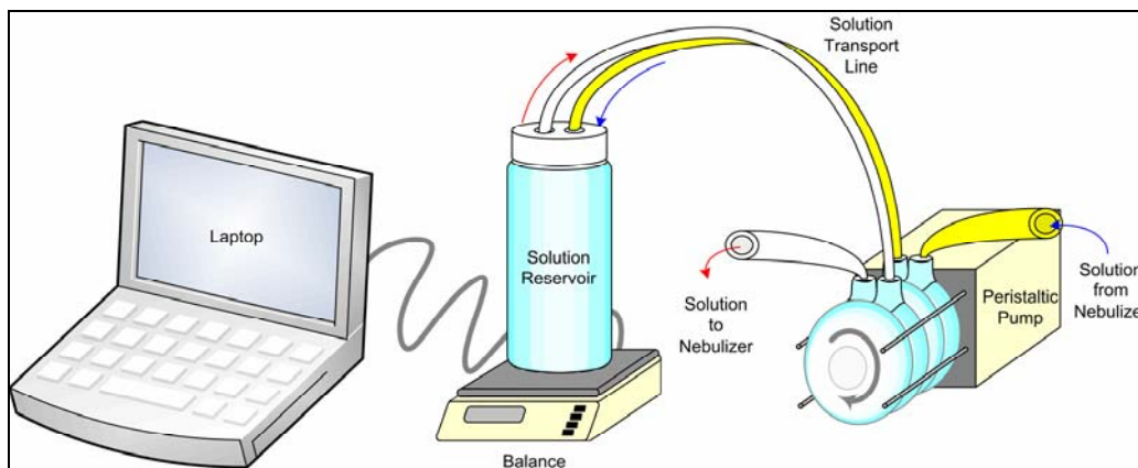
Figure 2: Schematic of the CES QAG standard solution control system.
