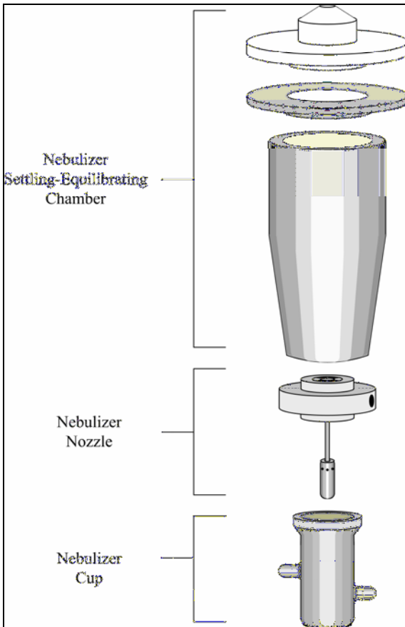
Figure 4: Schematic of the CES QAG nebulizer and droplet size control system.
