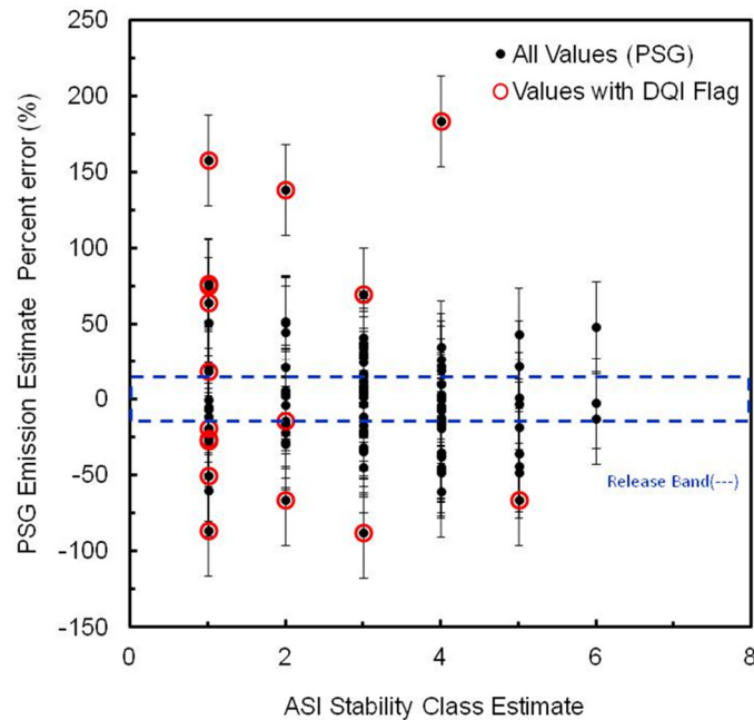
Figure 9-6. Summary of release trials by ASI
