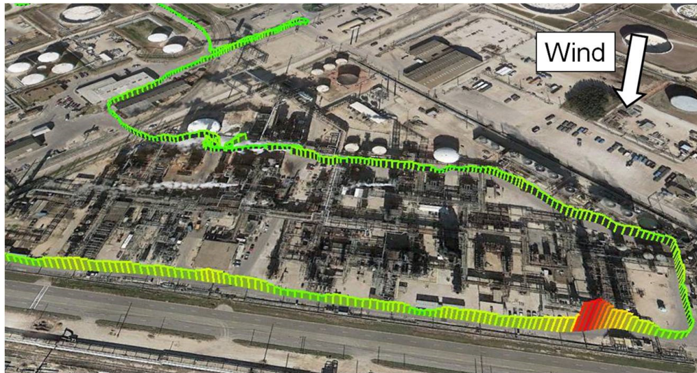
Figure 2-2. GMAP-REQ-DA concentration mapping survey of an industrial facility. Red points indicate elevated benzene levels
