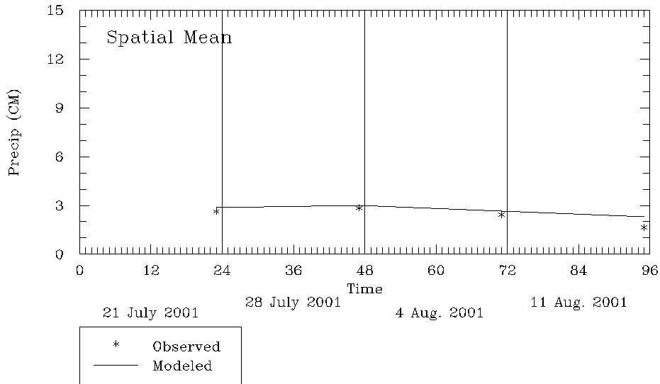
Neighborhood Spatial Mean 36km in the MW
