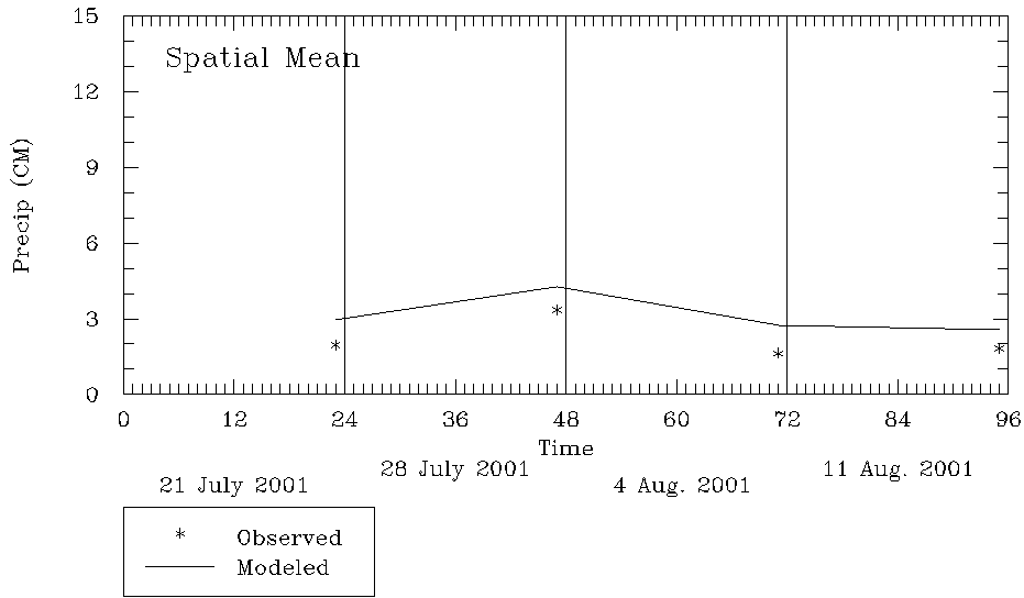
Neighborhood Spatial Mean 36km in the CENRAP
