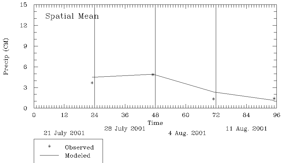
Neighborhood Spatial Mean 12km in the WRAP
