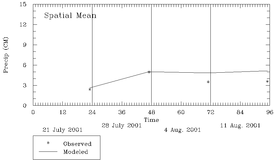
Neighborhood Spatial Mean 36km in the VISTAS
