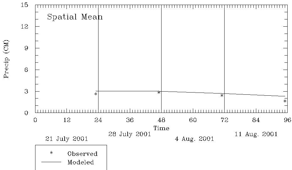
Neighborhood Spatial Mean 12km in the MW
