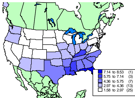
Figure 3-171: Annual Accumulated Mean Precipitation Error (cm).
