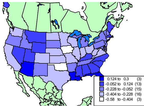
Figure 3-125: Episode Average Mixing Ratio Bias (g/kg).
