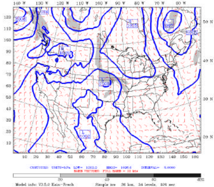
Surface data plot for 12Z 30 MAY 01
