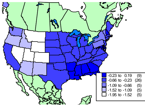
Figure 3-81: Episode Average Temperature Bias (Deg. C).
