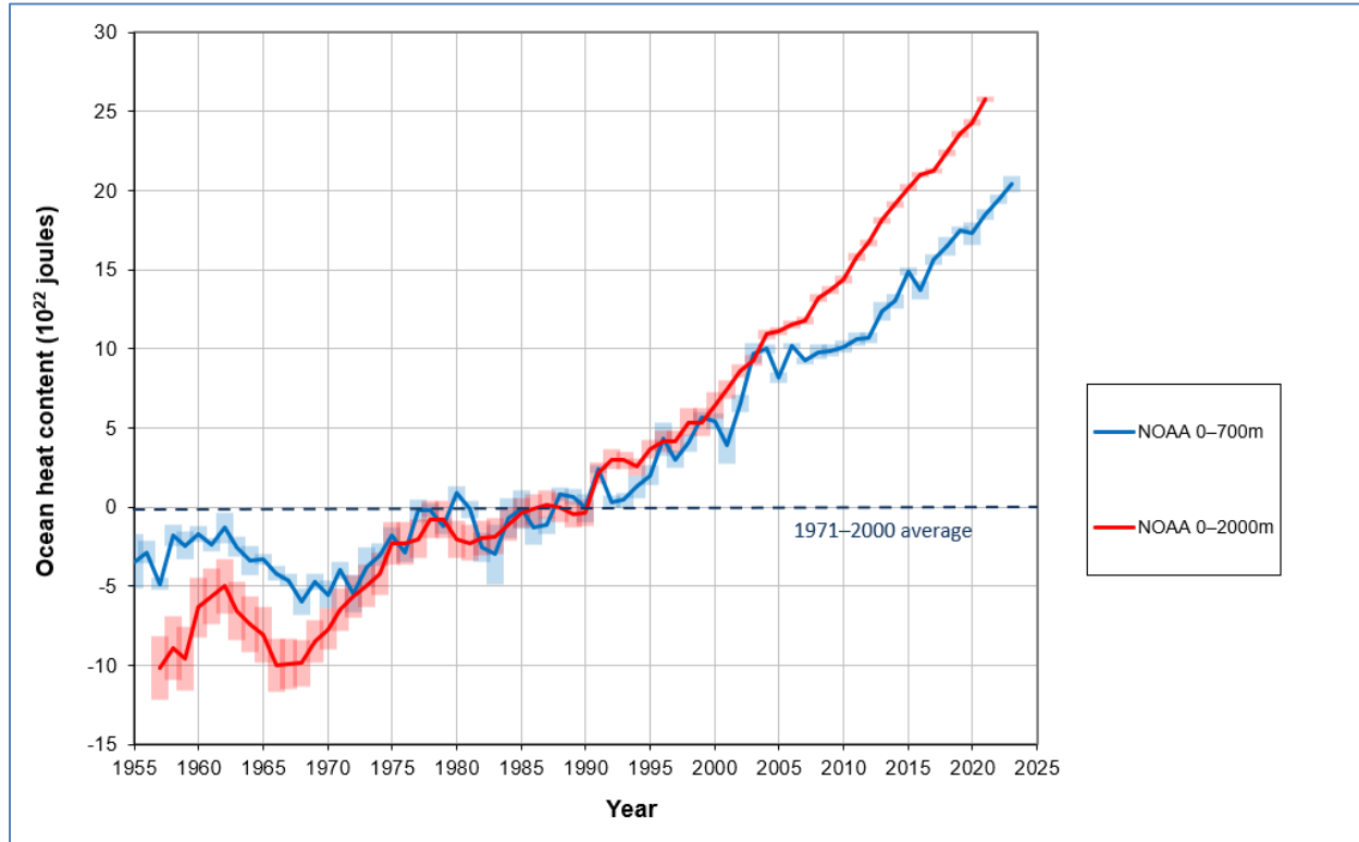
Figure TD-5. Ocean Heat Content in the Top 700 Meters and the Top 2,000 Meters in the NOAA Data Sets, 1955–2023, with Standard Errors
