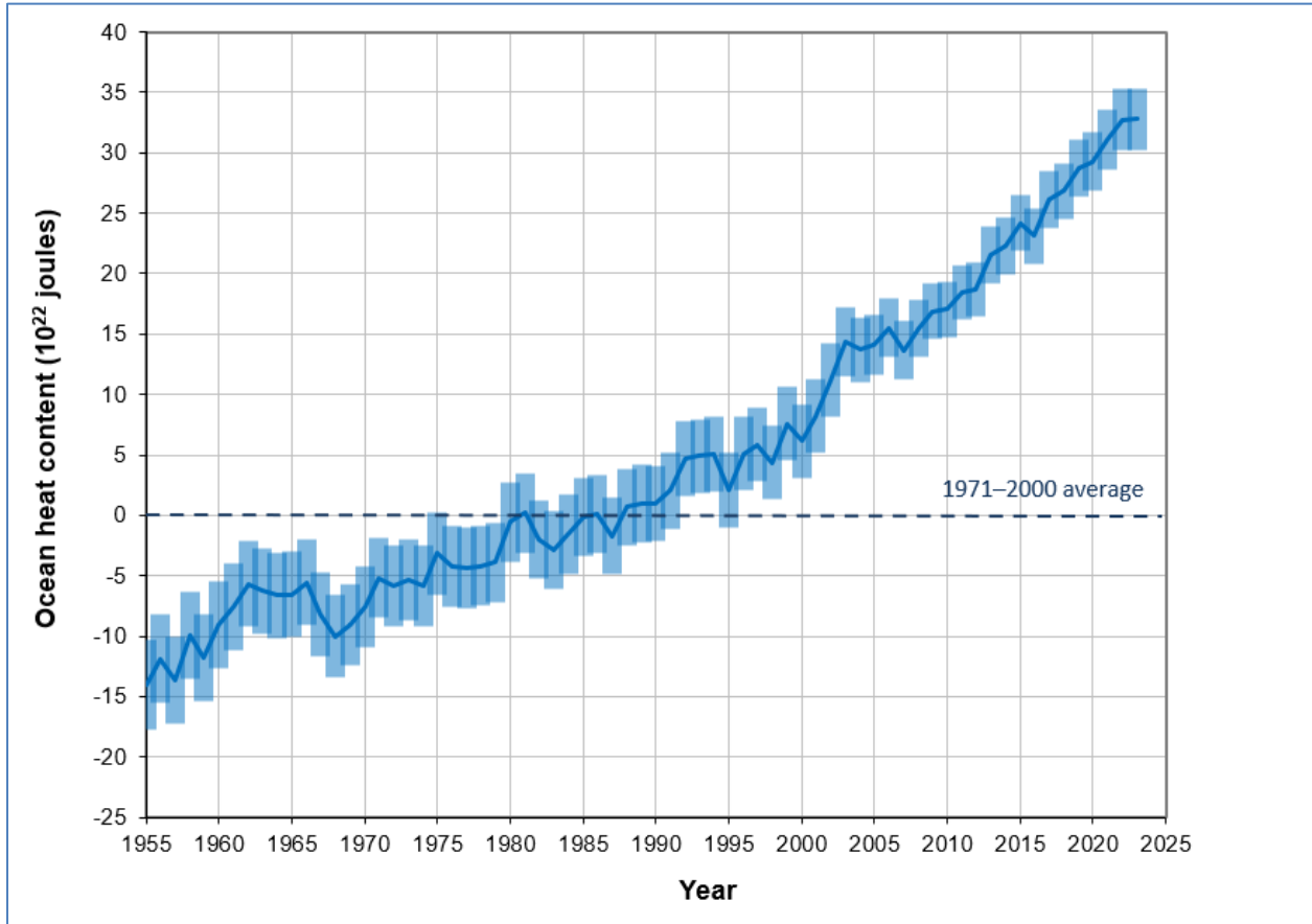
Figure TD-4. Ocean Heat Content for the Top 2,000 Meters from the MRI/JMA Data Set, 1955–2023, with 95 Percent Confidence Intervals
