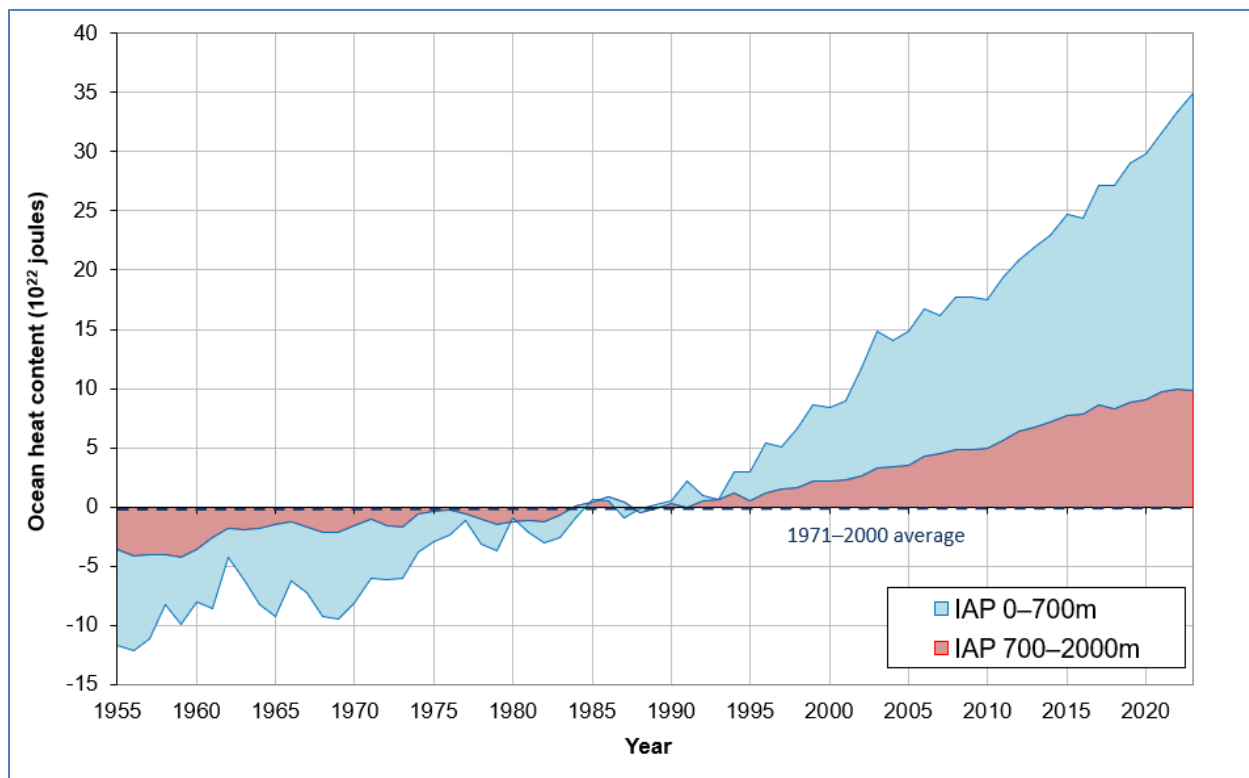
Figure TD-1. Relative Contributions to Changes in Ocean Heat Content in the IAP Data Set, by Depth, 1955–2023
