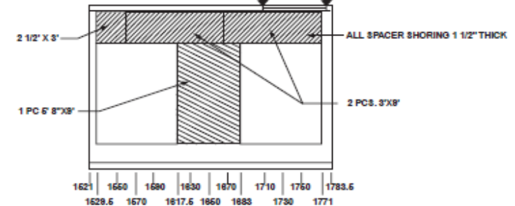
CENTER LOWER COMPARTMENT ALL MODELS CARGO DOOR W/483L PALLET / SHORING 70 X 88
