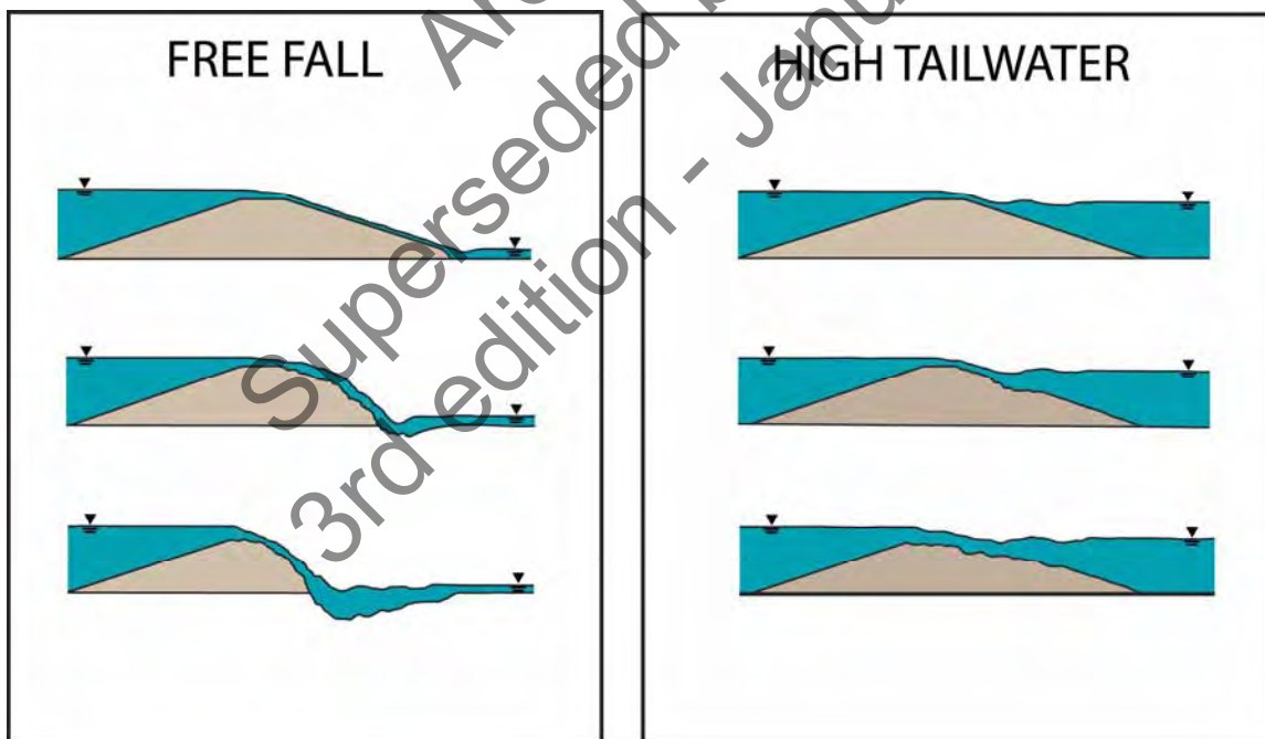
Figure 8.5. Embankment failure mechanisms (after Clopper and Chen 1988)
