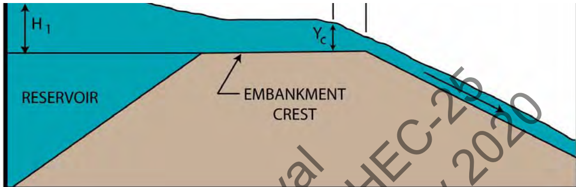
Figure 8.4. Flow regimes leading to failure of embankments in riverine flooding situations (after Clopper and Chen 1988).
