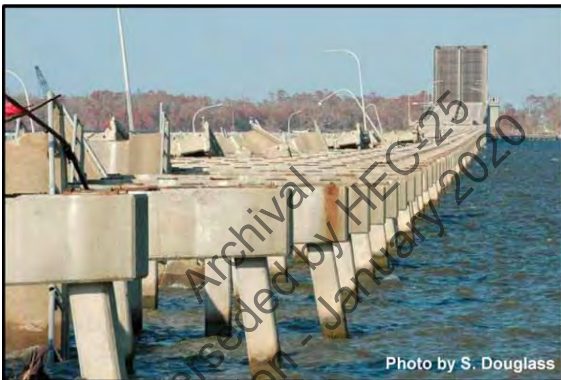
Figure 2.5. US Highway 90 bridge across Biloxi Bay, Mississippi, after Hurricane Katrina. (photo looking northeast from Biloxi 9/21/05).
