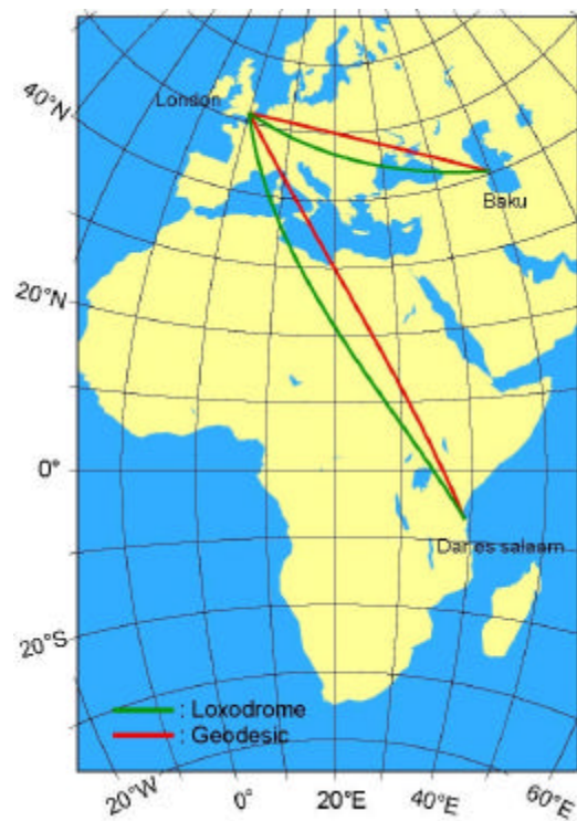
TRANSVERSE MERCATOR
