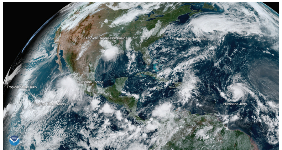
GOES-16 view of the Eastern Pacific and Atlantic Hurricane Basins on September 19. Credit: NOAA/CIRA
