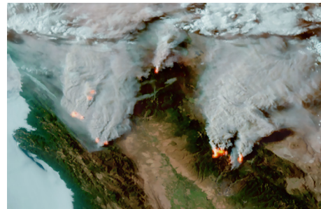
GOES-17 imagery of several large fires in northern California on Aug. 4, 2021. Credit: NOAA
