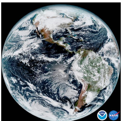
GOES-16 GeoColor full disk image taken Jan. 15, 2017.
