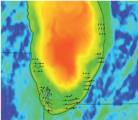
Ice along the southern Lake Michigan shoreline (denoted by arrows) on February 14, 2018, contrasts with the warmer, unfrozen lake water in this GOES-16 infrared imagery. Using a pair of images three hours apart, the ice motion code detected strong eastern/northeastern motion along the lakeshore. Some features were tracked moving more than 10 km in three hours. Credit: NOAA
