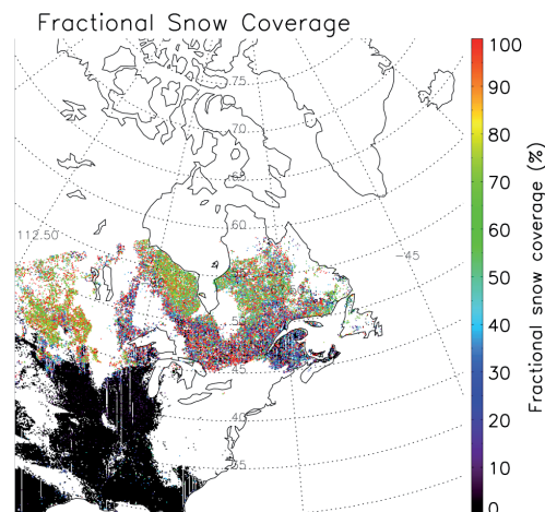
GOES-16 snow cover retrieval on March 21, 2018, which shows high fractional snow cover north and west of the Great Lakes, and snow-free land south of the Great Lakes. There are no fractional snow cover retrievals over areas east of the Great Lakes and elsewhere due to cloud cover. Credit: NOAA
