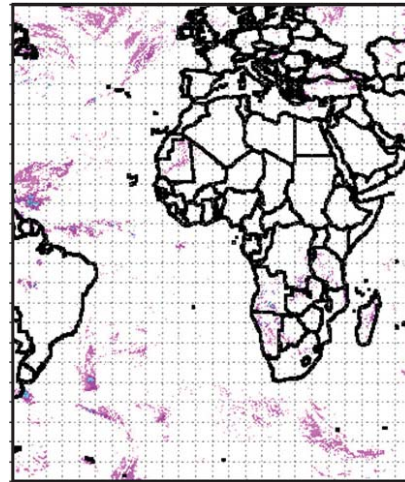
Example of the Rainfall Rate product as generated by the GOES-R Rainfall Rate algorithm using Meteosat-8/SEVIRI (Spinning Enhanced Visible and Infrared Imager) data on January 7, 2005 12:45 UTC. Credit: NOAA/NESDIS/STAR
