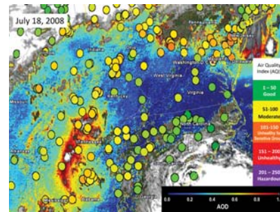
Values of Aerosol Optical Depth observed by GOES correlate well with EPA surface monitors (circles). GOES visible band observations were used to derive the Aerosol Optical Depth/Thickness. Credit: NOAA/NESDIS/STAR
