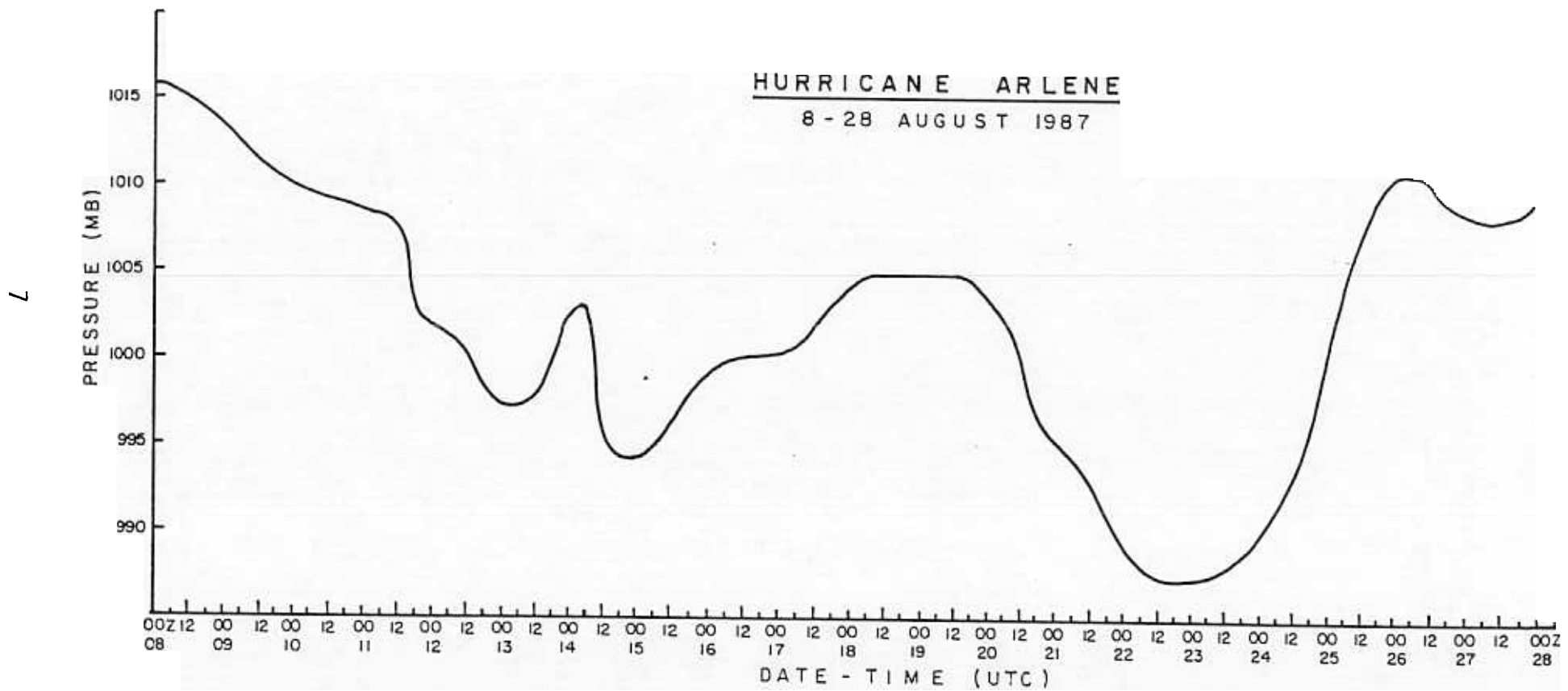
Figure 2. Lowest pressure vs. time, 1987 tropical cyclones.
