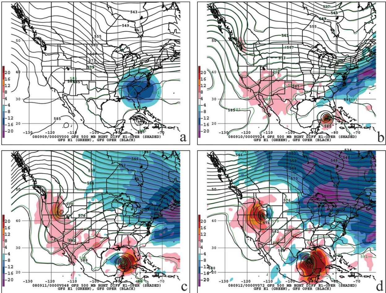
FIG. 12. GFS 500-hPa geopotential height (contours, dam) from the operational run (black) and perturbation experiment e1 (green) initialized at 0000 UTC 9 Sep 2008, and difference field e1-operational (shaded, m) for (a) the analysis, and (b) 24-, (c) 48-, and (d) 72-h forecasts.
