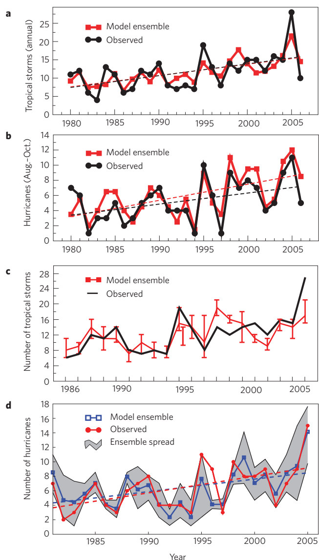
Figure 3 | Simulated versus observed Atlantic tropical cyclone interannual variability (approximately 1980–2006) using several methods.
