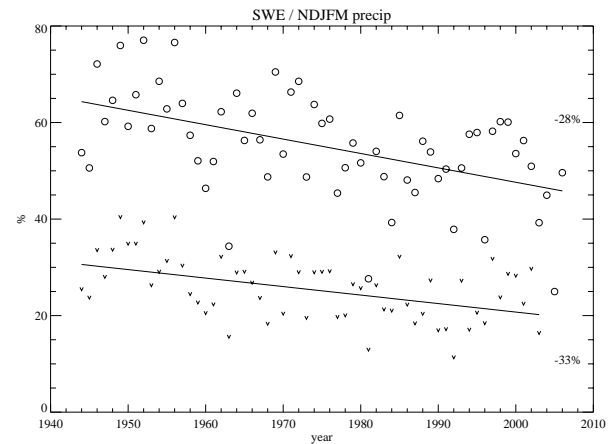
Fig. 8. “Storage efficiency,” the ratio of 1 April SWE to November–March precipitation, with linear fit, for observations (○) 1944–2006 and VIC (▼) simulation 1944–2003. The average storage efficiency in VIC is lower because the domain includes a lot of low-elevation grid points, but the percentage changes are similar.
