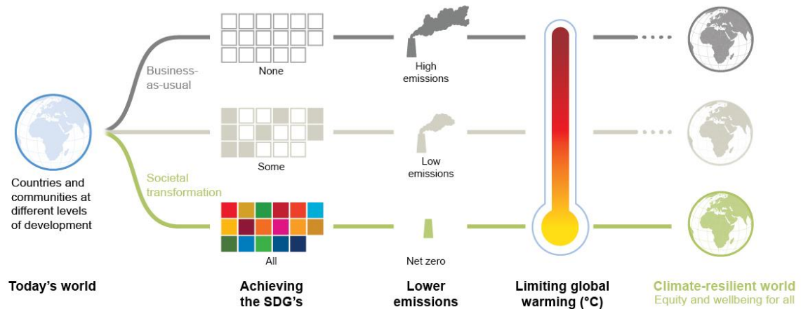
FAQ 5.2, Figure 1: Climate-resilient development pathways (CRDPs) describe trajectories that pursue the dual goal of limiting warming to 1.5°C while strengthening sustainable development. Decision-making that achieves the SDGs, lowers greenhouse gas emissions and limits global warming could help lead to a climate-resilient world, within the context of enhancing adaptation.
