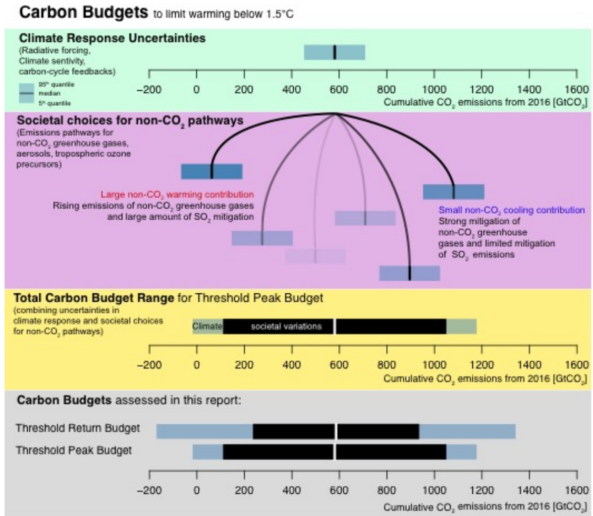
Figure SPM 4: Summary of the various uncertainties affecting carbon budget size for holding warming below 1.5°C relative to preindustrial levels from the 1 st January 2016 onwards. For threshold peak budget best estimate of 580 GtCO 2 as given in Table SPM 1, the climate response uncertainties associated to this budget are represented by the 5%-95% confidence interval inferred from outcomes due to variation of geophysical parameters in the simple climate model setup used for this assessment. Uncertainties in climate response include those associated to radiative forcing, climate sensitivity, and carbon-cycle feedbacks. Societal choices influencing the carbon budget size are related to societal variations for non-CO 2 forcing which are illustrated by the full range of forcing futures found in the integrated pathways available in the SR1.5 scenarios database. A “large non-CO 2 warming contribution” represents 0.85 W m -2 of non-CO 2 radiative forcing at the time of deriving the carbon budget, a “small non- CO 2 cooling contribution” represents -0.02 W m -2 of non-CO 2 radiative forcing. The median non- CO 2 radiative forcing estimate across all available pathways is 0.45 W m -2 of non-CO 2 radiative forcing. The total carbon budget range provides an overview of the combined uncertainties in threshold peak budget due to the aforementioned factors. Median threshold peak budgets and threshold return budgets as given in Table SPM 1 are indicated by the vertical bold white line in the bottom panel.
