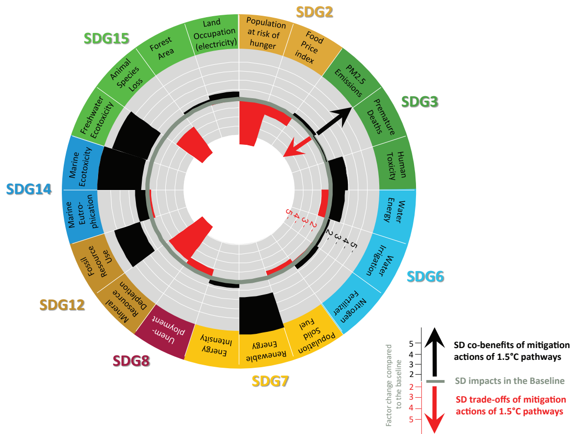
Figure SPM 6: Co-benefits (black) and risks for trade-offs (red) of mitigation consistent with limiting mean temperature to 1.5°C by 2100 assuming middle-of-the-road future socio-economic development. Co-benefits and trade-offs are measured in 2050 relative to middle-of-the-road baseline pathways without new mitigation policies (bold grey circle), and cover 21 sustainable development dimensions across seven Sustainable Development Goals (SDGs) (and selected sub-targets). Range denotes estimates across six different integrated assessment models, which were coupled to disciplinary models for the assessment of hunger, health, energy access, toxicity, and mineral resource implications of the pathways. Note that the realization of the side-effects will critically depend on local circumstances and implementation practice. Trade-offs across many SD dimensions can be eradicated through complementary/redistributional measures. Figure is not comprehensive and focuses on SD dimensions for which quantifications across models are available.
