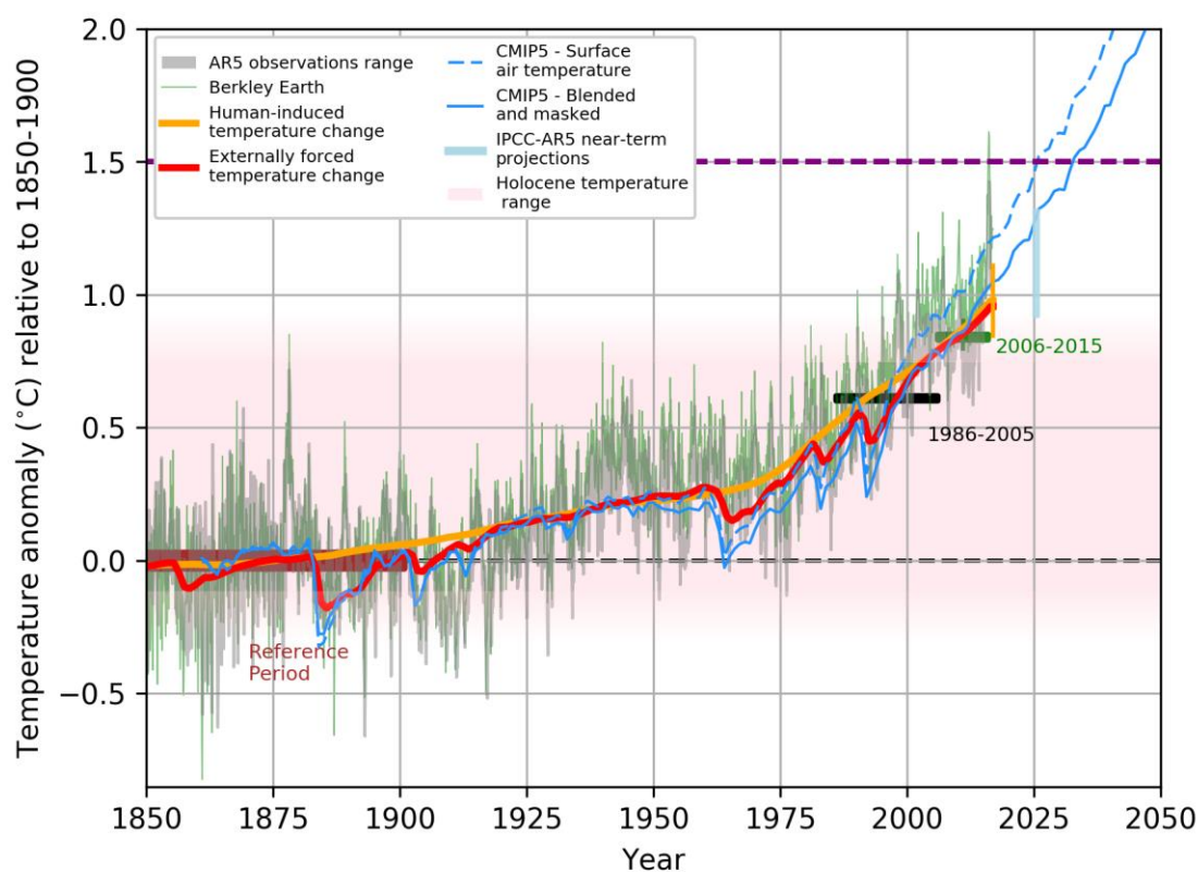
Figure 1.2: Evolution of global mean surface temperature (GMST) over the period of instrumental observations. Grey line shows departures from the 1850–1900 reference period for monthly means of the HadCRUT4, NOAA and GISTEMP datasets assessed in AR5, with line thickness indicating inter–dataset range. Green line shows the Berkeley Earth Surface Temperature as an example of more recent datasets using statistical methods to further account for the impact of incomplete coverage. All observational datasets shown represent GMST as a blended mix of near surface air temperature over land and sea surface temperature over oceans. Human–induced (orange) and total human– and naturally–forced (red) contributions to these GMST changes are shown calculated following Otto et al. (2015) and Haustein et al. (2017). Proportional uncertainty in the level of human–induced warming in 2016 is set equal to that assessed in Bindoff et al. (2013). Thin blue lines show the modelled global–mean surface air temperature (dashed) and blended surface air and sea surface temperature accounting for observational coverage (solid) from the CMIP5 ensemble under the Historical and RCP8.5 scenario (Cowtan et al., 2015; Richardson et al., 2016). The pink shading indicates a range for temperature fluctuations over the Holocene (Marcott et al., 2013; Marsicek et al., 2017). Near–term predictions for global mean warming for the 2016–2035 period from Kirtman et al. (2013) are shown in light blue. See Technical Annex 1.A of this chapter for further details.
