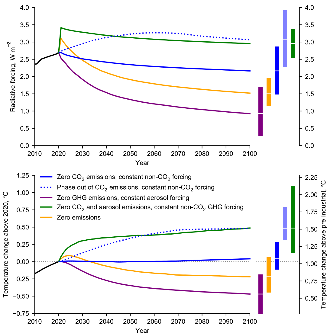
18 Figure 1.6: Radiative forcing (top) and global mean surface temperature change (bottom) for scenarios with 19 different combinations of greenhouse gas and aerosol precursor emissions reduced to zero in 20 2020. Variables were calculated using a simple climate-carbon cycle model (Millar et al., 2017b) 21
