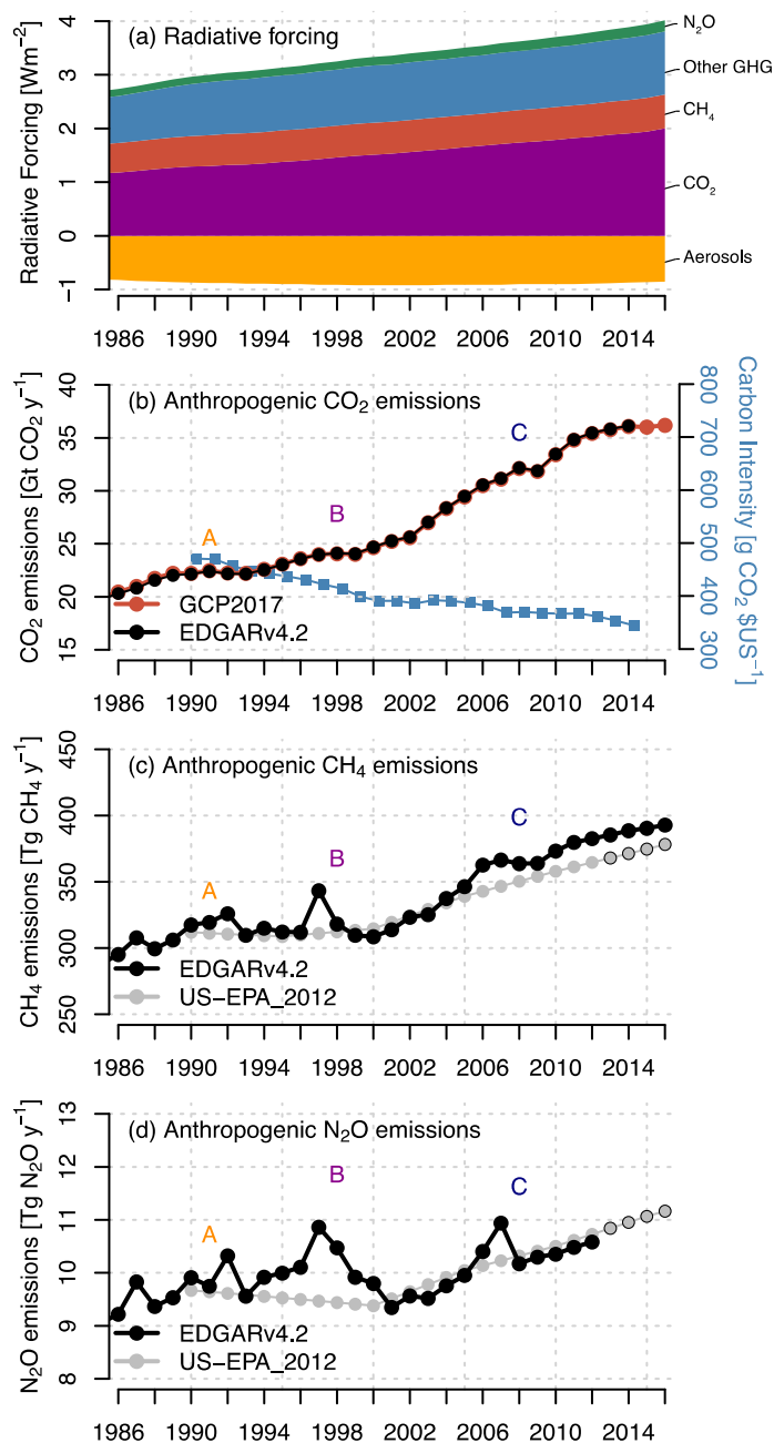
11 Figure 1.4: Time series of anthropogenic radiative forcing (a), CO 2 , methane (CH 4 ) and nitrous oxide (N 2 O) 12 emissions (b–d) for the period 1986–2016. Anthropogenic radiative forcing is estimated according to 13 Etminan et al. (2016) using Dlugokencky and Tans (2016) for greenhouse gases concentrations 14 and ECLIPSE data for aerosols. Anthropogenic CO 2 emissions are from the Global Carbon
