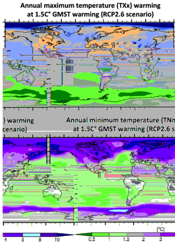
Figure S3.4 Same analysis as left-hand part of Fig. 3.5 but based on RCP2.6 scenario CMIP5 simulations
