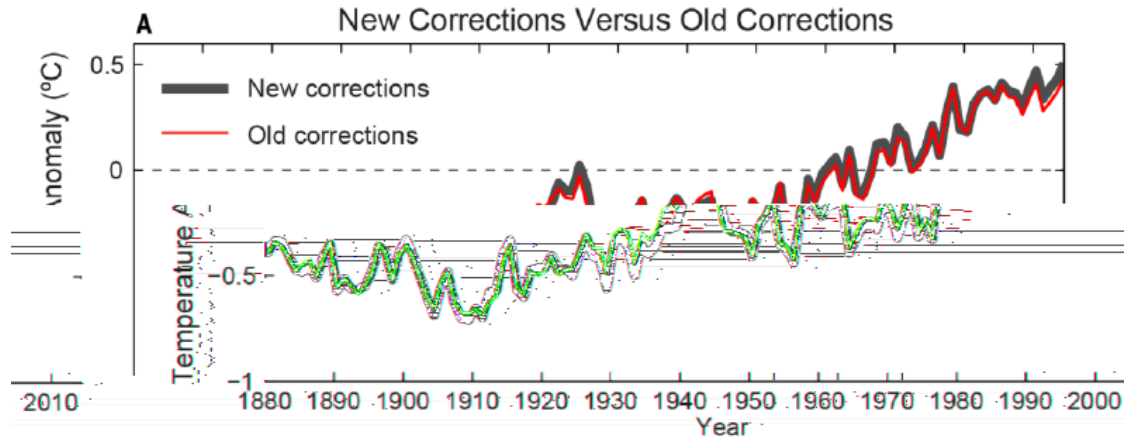
Figure S3.2 Global temperature warming using older and newer corrections (Karl et al. 2015)
