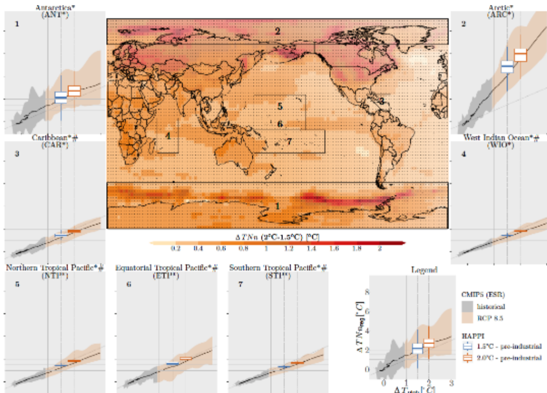
Figure 3.SM.10: Same analysis as Figure S3.8 (projected changes in annual minimum nighttime temperature (TNn) as function of global temperature warming) for additional regions displayed with asterisks in Figure 3.2 (island regions, polar regions). Asterisks (*) indicate non-SREX reference regions ( http://www.ipcc-data.org/guidelines/pages/ar5_regions.html ). Pound sign (#) indicates island regions; for these regions, the ocean area was not masked out in the analyses.
