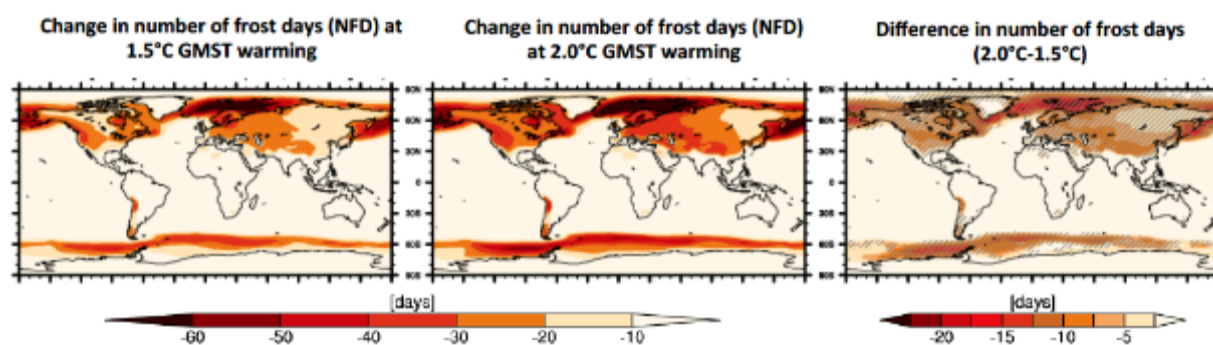
Figure 3.SM.13: Projected changes in number of hot days (10% warmest days, top) and in number of frost days (days with T < 0^\circ\text{C} , bottom) at 1.5°C (left) and 2°C (right) GMST warming, and their difference (right; hatching highlights areas in which 2/3 of the models agree on the sign of change). Adapted from Wartenburger et al. (2017).
