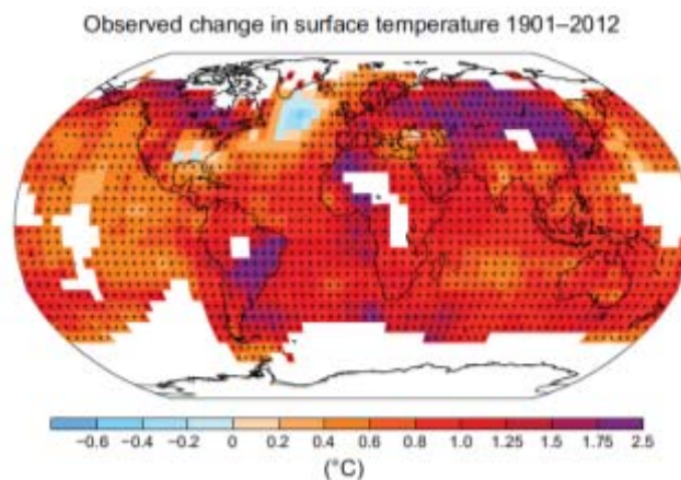
Figure 3.SM.1: Map of the observed surface temperature change from 1901 to 2012 derived from temperature trends determined by linear regression from one dataset. Trends have been calculated where data availability permits a robust estimate (i.e., only for grid boxes with greater than 70% complete records and more than 20% data availability in the first and last 10% of the time period). Other areas are white. Grid boxes where the trend is significant at the 10% level are indicated by a + sign. From Stocker et al. (2013).
