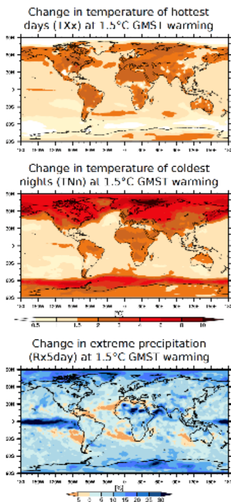
Figure 3.SM.5: Same as left-hand plot of Figure 3.4, but based on the Representative Concentration Pathway (RCP)2.6 scenarios
