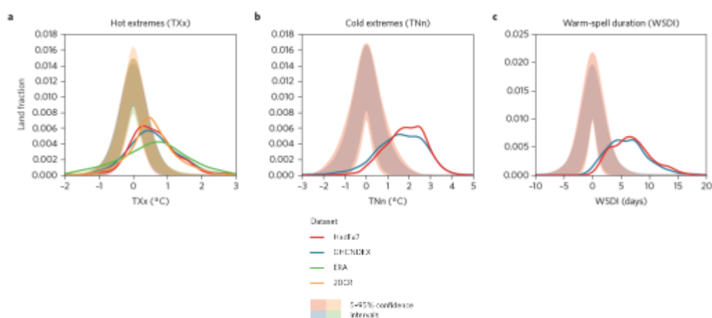
Figure 3.SM.6: Difference in extreme temperature event indices for 0.5°C warming over the observational record. Probability density functions show the globally aggregated land fraction that experienced a certain change between the 1991–2010 and 1960–1979 periods for the HadEX2 and GHCNDEX datasets. For TXx, the analysis includes also reanalysis data from the European Centre for Medium-Range Forecasts (ECMWF) (ECMWF Reanalysis 40 (ERA-40) and Interim (ERA-Interim), used as a combined dataset including ERA-40 until 1979 and ERA-Interim from
