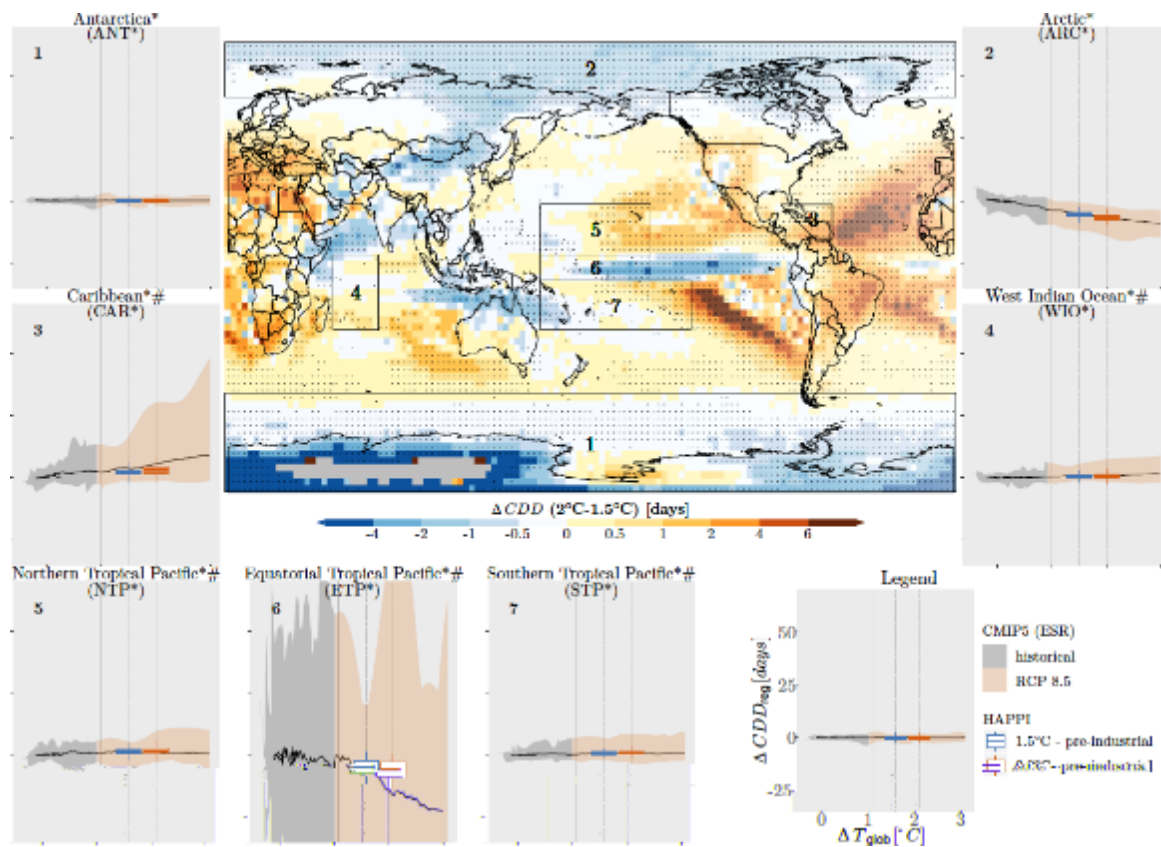
Figure 3.SM.15: Same analysis as Figure 3.12 for additional regions displayed with asterisks in Figure 3.2 (island regions, polar regions). Asterisks (*) indicate non-SREX reference regions ( http://www.ipcc-data.org/guidelines/pages/ar5_regions.html ). Pound sign (#) indicates island regions; for these regions, the ocean area was not masked out in the analyses.
