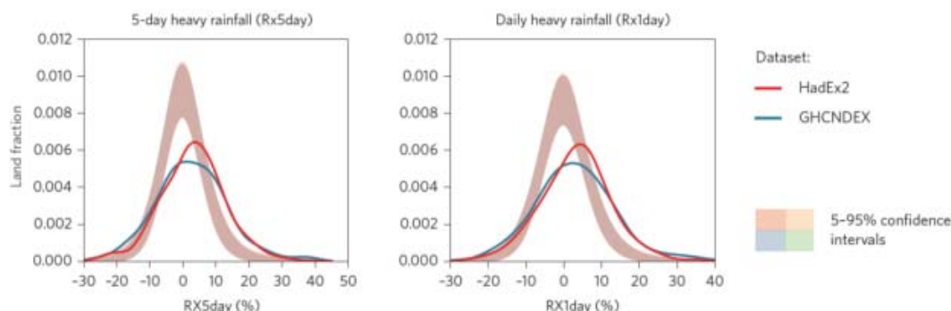
Figure 3.SM.7: Differences in extreme precipitation event indices for 0.5°C warming over the observational record. Probability density functions show the globally aggregated land fraction that experienced a certain change between the 1991–2010 and 1960–1979 periods for the HadEX2 and GHCNDEX datasets. Light-coloured envelopes illustrate the changes expected by internal variability alone, estimated by statistically resampling individual years. From Schleussner et al. (2017)
