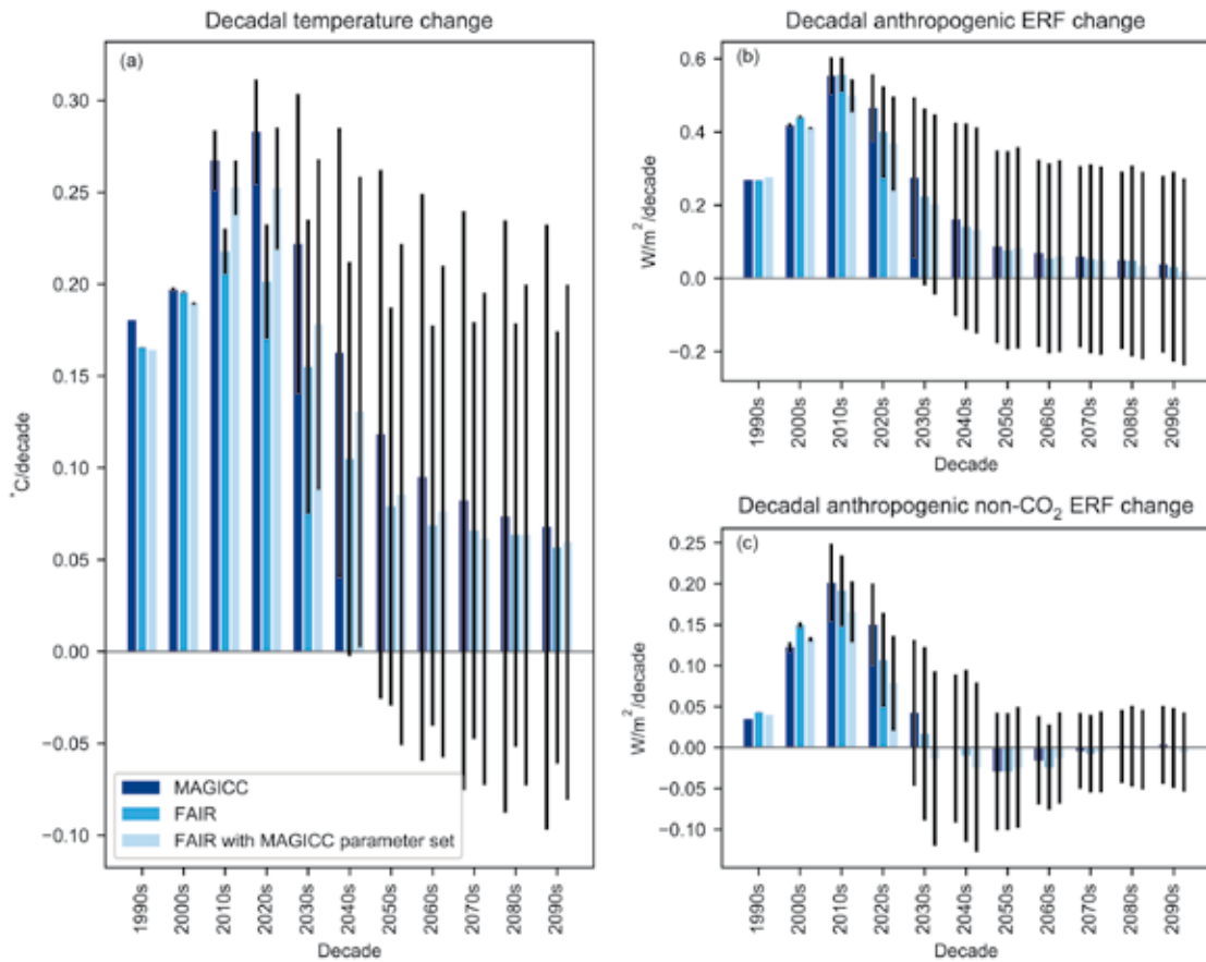
Figure 2.SM.1 | Warming rates per decade for MAGICCC (dark blue), FAIR (sky blue) and FAIR matching the MAGICCC parameter set (light blue) for the scenario dataset used in this report. These bars represent the mean of regression slopes taken over each decade (years 0 to 9) for scenario median temperature changes, over all scenarios. The black bars show the standard deviation over the set of scenarios.
