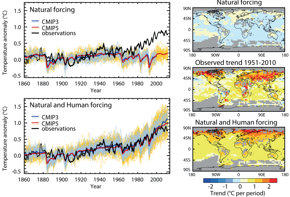
Figure 3.SM.3 | Attribution of global warming change (from IPCC AR5, Bindoff et al., 2013a)
