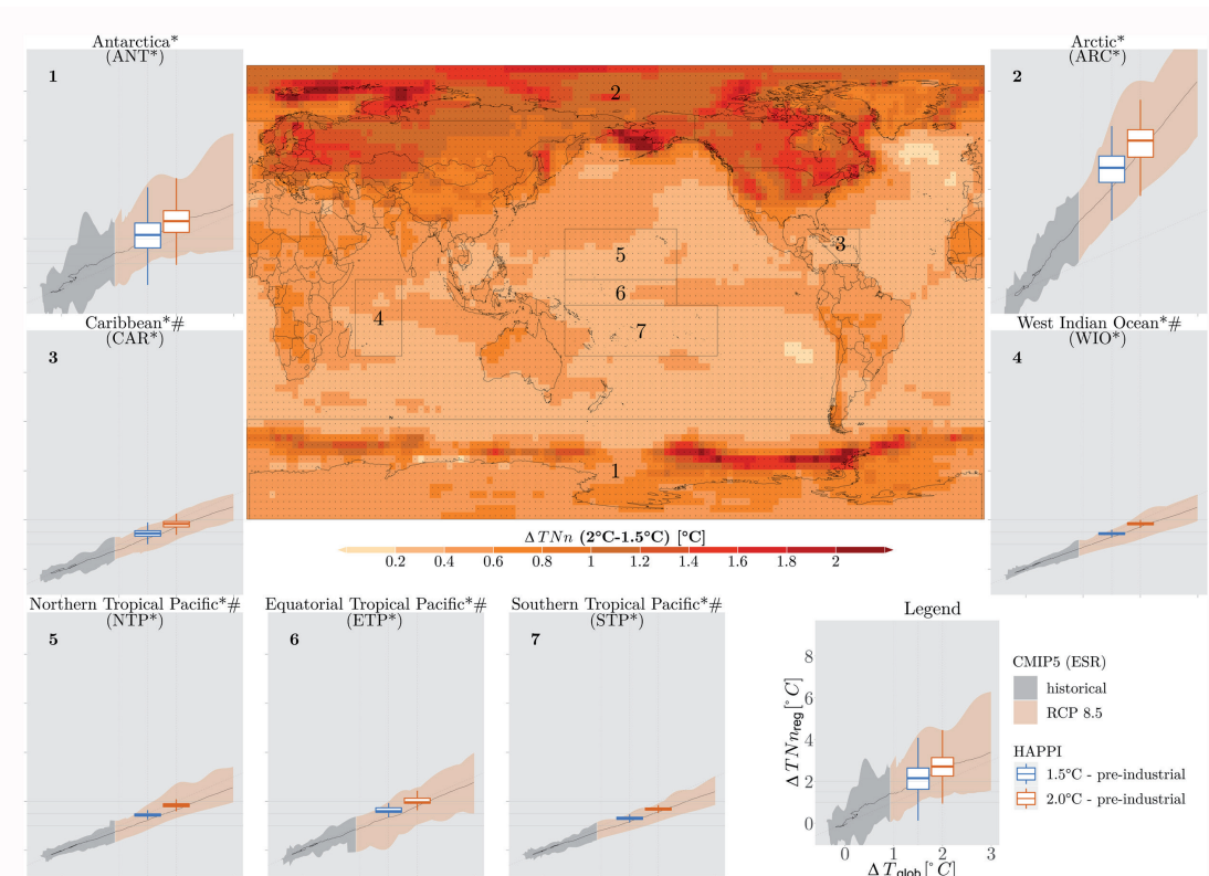
Figure 3.SM.10 | Same analysis as Figure S3.8 (projected changes in TNn as function of global temperature warming) for additional regions displayed with asterisks in Figure 3.2 (island regions, polar regions). Asterisks (*) indicate non-SREX reference regions ( http://www.ipcc-data.org/guidelines/pages/ar5_regions.html ). Hashtag (#) indicates island regions; for these regions, the ocean area was not masked out in the analyses.
