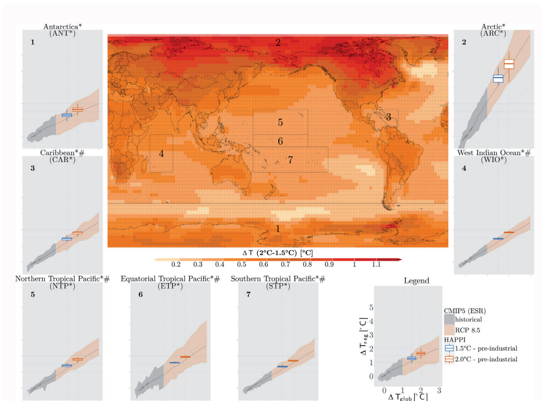
Figure 3.SM.12 | Same analysis as Figure 3.SM.11 (projected in the changes in Tmean as function of the mean global temperature) for additional regions displayed with asterisks in Figure 3.2 (island regions, polar regions). Asterisks (*) indicate non-SREX reference regions ( http://www.ipcc-data.org/guidelines/pages/ar5_regions.html ). Hashtag (#) indicates island regions; for these regions, the ocean area was not masked out in the analyses.
