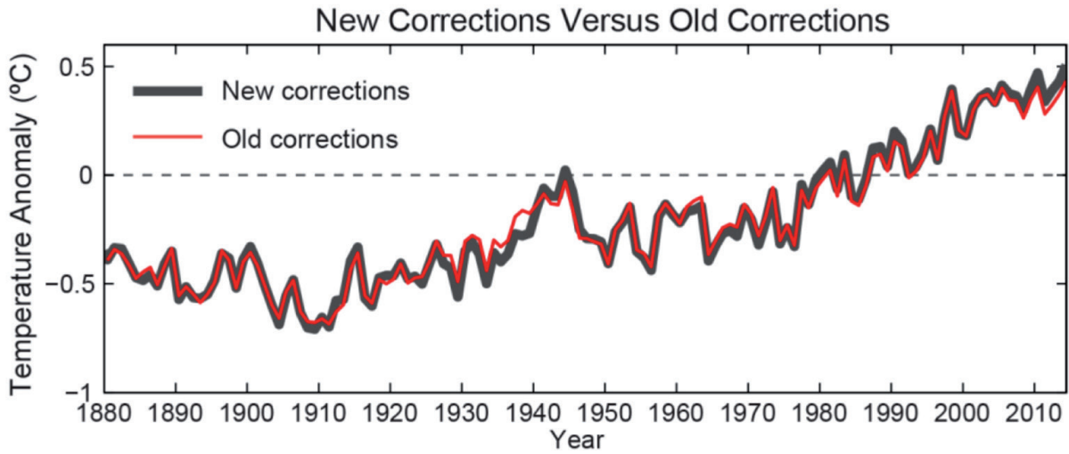
Figure 3.SM.2 | Global temperature warming using older and newer corrections (Karl et al., 2015).
