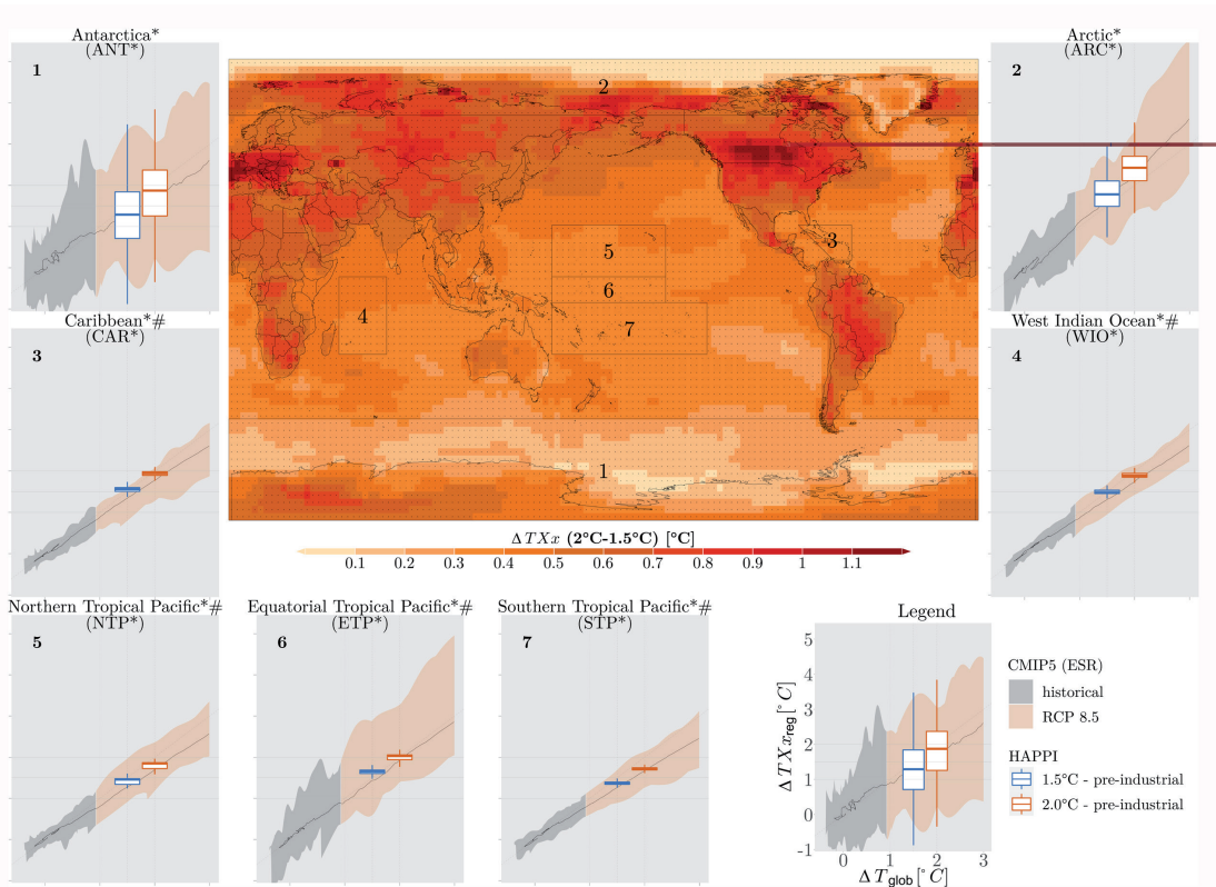
Figure 3.SM.9 | Same analysis as Figure 3.5 (projected changes in annual maximum value of daily maximum temperature, TXx, as function of global temperature warming) for additional regions displayed with asterisks in Figure 3.2 (island regions, polar regions). Asterisks (*) indicate non-SREX reference regions ( http://www.ipcc-data.org/guidelines/pages/ar5_regions.html ). Hashtag (#) indicates island regions; for these regions, the ocean area was not masked out in the analyses. See description of computation of Figure 3.5 in the present Annex for more details.
