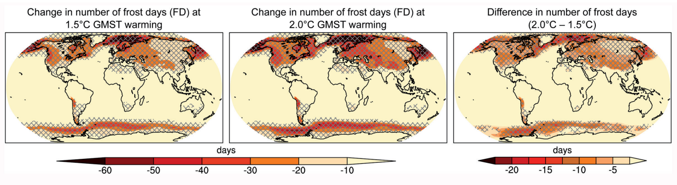
Figure 3.SM.13 | Projected changes in number of frost days (days with T < 0^{\circ}\text{C} , bottom) at 1.5°C (left) and 2°C (middle) GMST increase, and their difference (right). Cross-hatching highlights areas in which at least 2/3rds of the models agree on the sign of change as a measure of robustness (18 or more out of 26). Adapted from Wartenburger et al. (2017).
