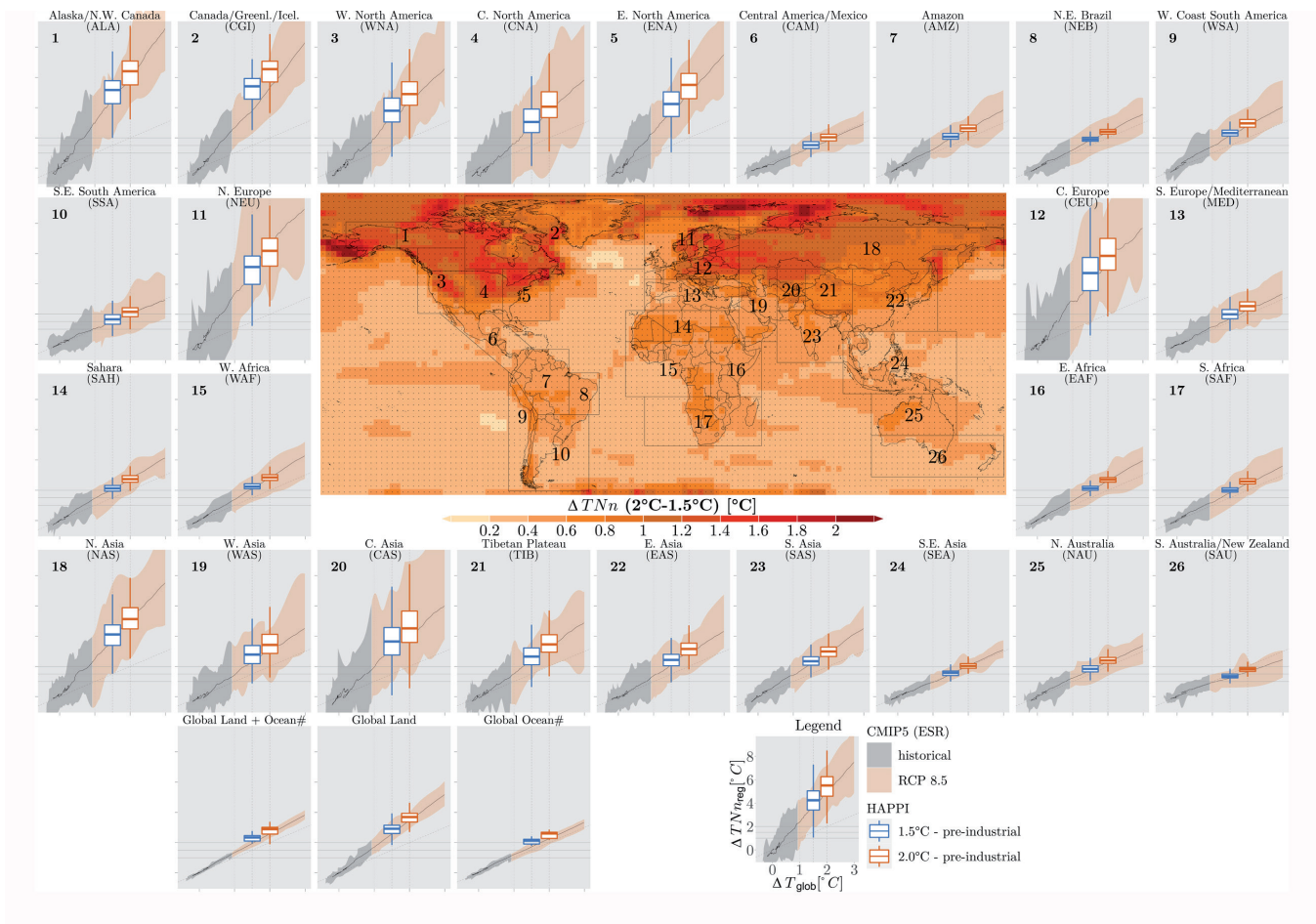
Figure 3.SM.8 | Same analysis as Figure 3.5, but for the annual minimum value of daily minimum temperature (T N ). For more details on computation, see description of computation of Figure 3.5 in the present Annex, as well as Wartenburger et al. (2017), Seneviratne et al. (2016) and Seneviratne et al. (2018).
