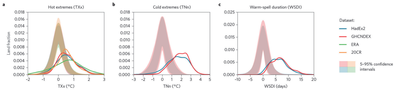
Figure 3.SM.6 | Difference in extreme temperature event indices for 0.5°C warming over the observational record. Probability density functions show the globally aggregated land fraction that experienced a certain change between the 1991–2010 and 1960–1979 periods for the Hadley Centre Global Climate Extremes Index 2 (HadEx2) and Global Historical Climatology Network (GHCN)-Daily climate Extremes (GHCNDEX) datasets. For annual maximum value of daily maximum temperature (TXx), the analysis also includes reanalysis data from the European Centre for Medium-Range Forecasts (ECMWF) (ECMWF Reanalysis 40 (ERA-40) and Interim (ERA-Interim), used as a combined dataset including ERA-40 until 1979 and ERA-Interim from 1979 onward) and the Twentieth Century Reanalysis (20CR) ERA and 20CR over the global land area. Light-coloured envelopes illustrate the changes expected by internal variability alone, estimated by statistically resampling individual years. From Schleussner et al. (2017).
