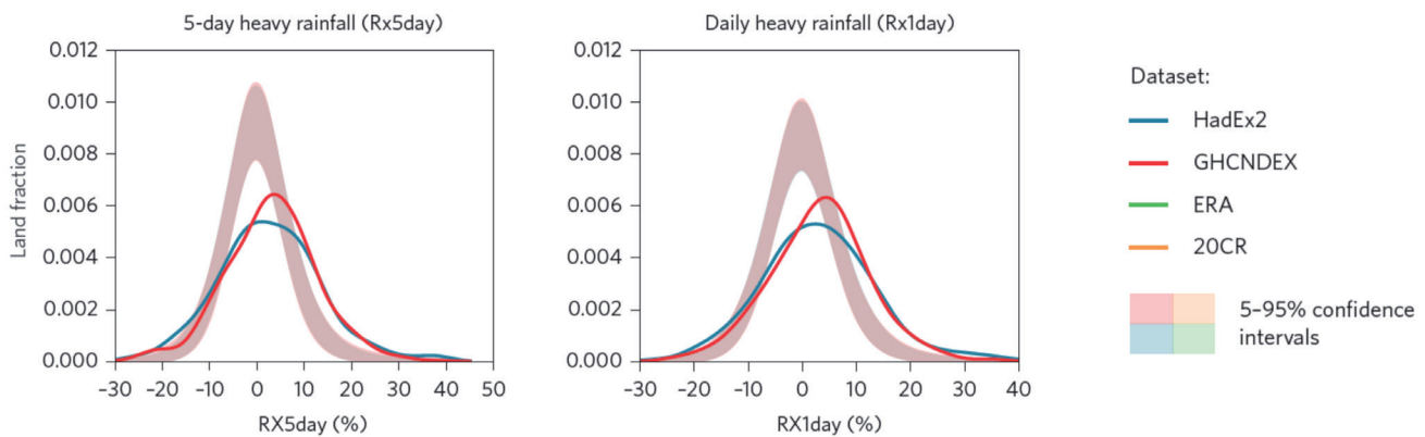
Figure 3.SM.7 | Differences in extreme precipitation event indices for 0.5°C warming over the observational record. Probability density functions show the globally aggregated land fraction that experienced a certain change between the 1991–2010 and 1960–1979 periods for the HadEx2 and GHCNDEX datasets. Light-coloured envelopes illustrate the changes expected by internal variability alone, estimated by statistically resampling individual years. From Schleussner et al. (2017).
