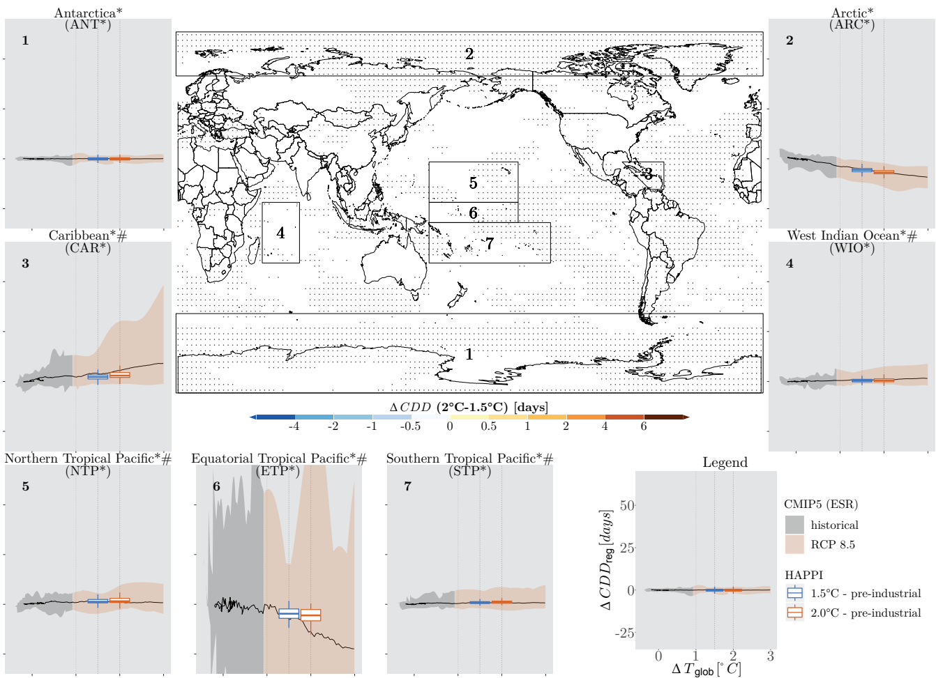
Figure 3.SM.15 | Same analysis as Figure 3.12 for additional regions displayed with asterisks in Figure 3.2 (island regions, polar regions). Asterisks (*) indicate non-SREX reference regions ( http://www.ipcc-data.org/guidelines/pages/ar5_regions.html ). Hashtag (#) indicates island regions; for these regions, the ocean area was not masked out in the analyses.
