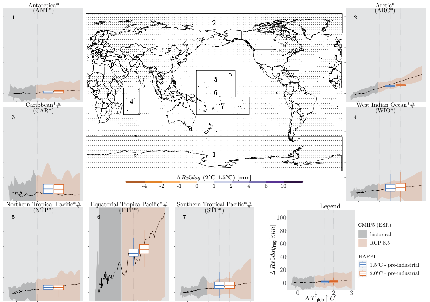
Figure 3.SM.14 | Same analysis as Figure 3.9 for additional regions displayed with asterisks in Figure 3.2 (island regions, polar regions). Asterisks (*) indicate non-SREX reference regions ( http://www.ipcc-data.org/guidelines/pages/ar5_regions.html ). Hashtag (#) indicates island regions; for these regions, the ocean area was not masked out in the analyses.
