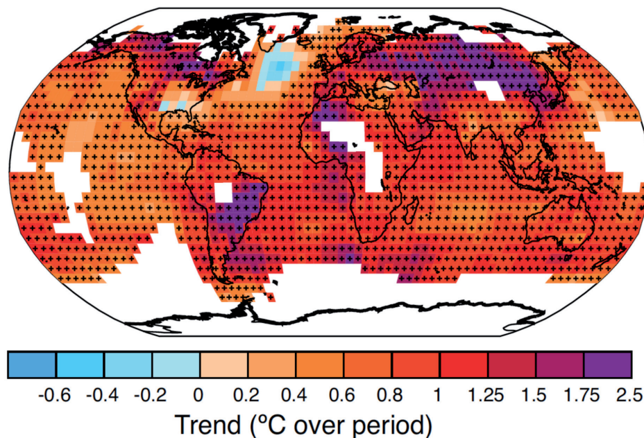
Figure 3.SM.1 | Map of the observed surface temperature change from 1901 to 2012 derived from temperature trends determined by linear regression from one dataset. Trends have been calculated where data availability permits a robust estimate (i.e., only for grid boxes with greater than 70% complete records and more than 20% data availability in the first and last 10% of the time period). Other areas are white. Grid boxes where the trend is significant at the 10% level are indicated by a + sign. From Stocker et al. (2013).
