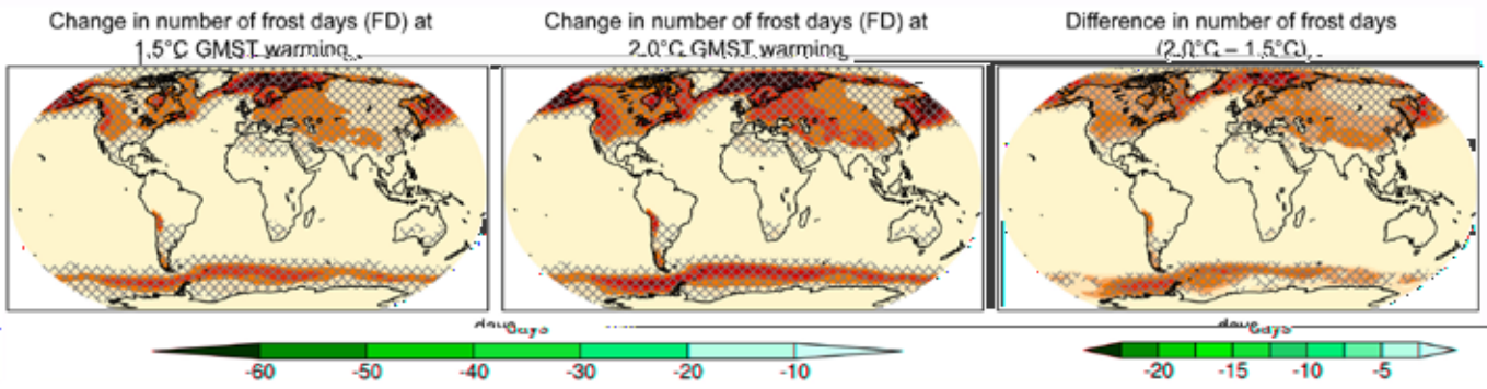
Figure 3.SM.13 | Projected changes in number of frost days (days with T < 0^\circ\text{C} , bottom) at 1.5°C (left) and 2°C (middle) GMST increase, and their difference (right). Cross-hatching highlights areas in which at least 2/3rds of the models agree on the sign of change as a measure of robustness (18 or more out of 26). Adapted from Wartenburger et al. (2017).
