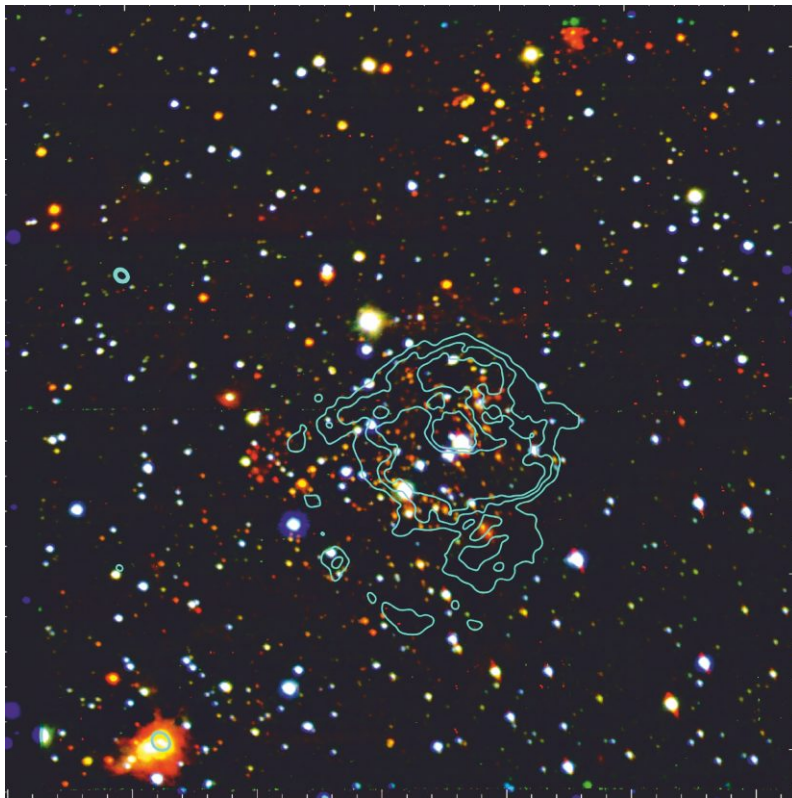
Figure 4: Colour composite image generated using data from ARIES 1.3m DFOT ( V -band, blue colour), 2m HCT-TRISPEC ( J -band: green, K band: red) overlaid with GMRT radio contour (1280 MHz) of the star forming region Sh2- 305, which is an HII region undergoing star formation due to impact of strong UV radiation from a nearby massive star. In the center is a young star cluster that is found to be embedded in a molecular cloud. The red sources are mostly embedded young stellar objects as seen from the deep K -band image that have formed mostly due to the impact of a strong UV radiation from a massive star (as seen by radio continuum contours). Figure credit: adapted from Pandey et al. 2020, Apj , 891, 81; Dewangan et al. 2020, ApJ , 898, 172
