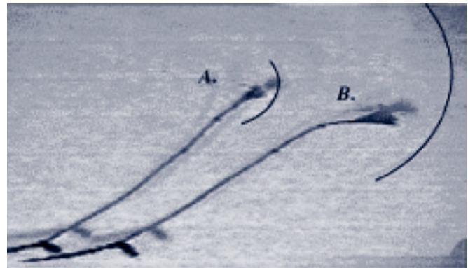
Figure 3: High-speed digital shadowgraphs of a cracking whip and its sonic boom. The time interval between the 2 pictures is 111µs. The solid lines are superimposed over the shock waves. The velocity at the time of the crack was Mach 2.19. (Photo courtesy of A. Krehl.)
