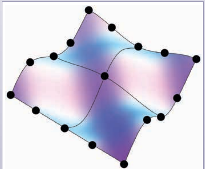
Figure B. Building a surface model via the serendipity finite element method: look up the terrain height only at perimeter grid points and at the central grid point.
