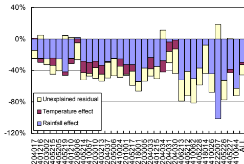
Figure 5: Proportion of observed streamflow reduction explained by streamflow sensitivity factors.
