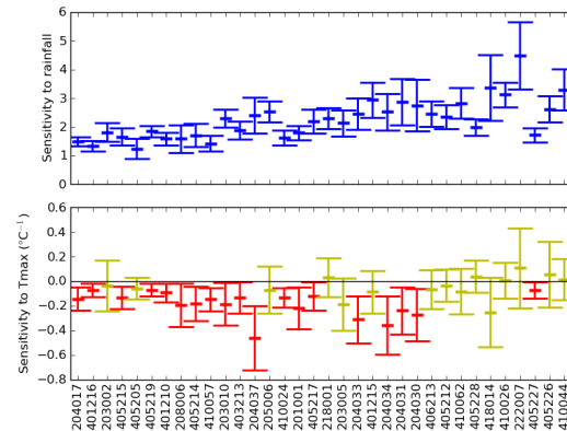
Figure 3: rainfall and temperature elasticities of streamflow ( \eta_P and \eta_T ). Mustard coloured ranges for \eta_T contain zero and are thus not statistically significant. Catchments are ordered by increasing dryness index.
