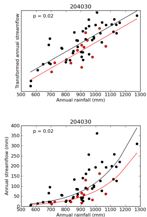
Figure 1: Testing the annual rainfall/streamflow relationship (catchment #204030 with maximum-likelihood Box-Cox parameter of 0.1). Red points and curves are for 1997–2008 data; black points and curves are for pre-1997 data.
