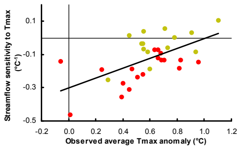
Figure 4: Relationship between streamflow sensitivity to Tmax and average Tmax anomaly during the drought (1997–2008 data compared to pre-1997 data).
