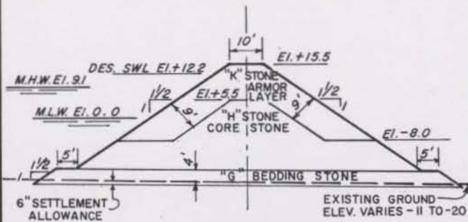
BREAKWATER TYPICAL SECTION SCALE IN FEET
