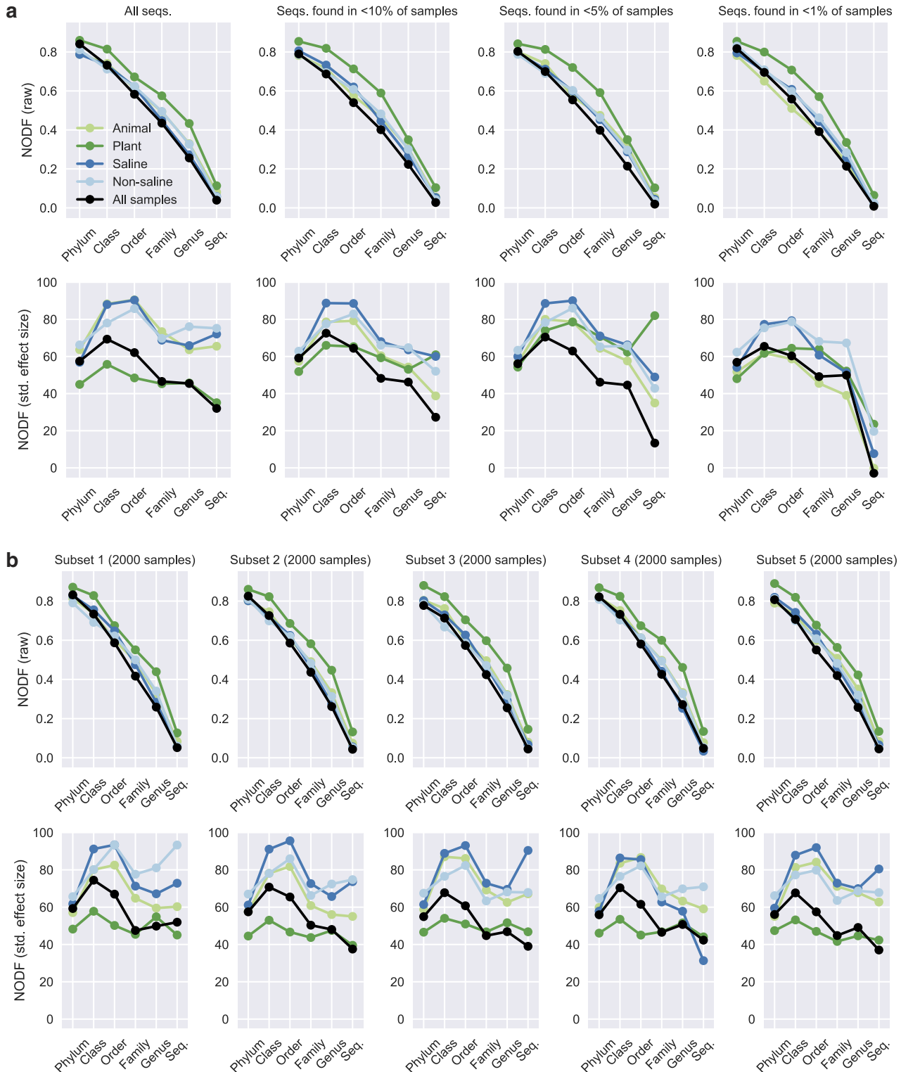
Extended Data Figure 6 | NODF scores of nestedness across samples by taxonomic level. The NODF statistic represents the mean, across pairs of samples, of the fraction of taxa occurring in less diverse samples that also occur in more diverse samples. A raw NODF of 0.5 would mean that for any pair of samples, on average 50% of the taxa in the less diverse sample would occur in the more diverse sample. a , NODF (raw) and NODF standardized effect size in the 2,000-sample subset by taxonomic level. Results are shown first for all tag sequences and then for tag sequences found in <10%, < 5%, and <1% of samples. By removing the most prevalent tag sequences before analysis (and rarefying only after this step), it was possible to rule out artefacts associated with potential
