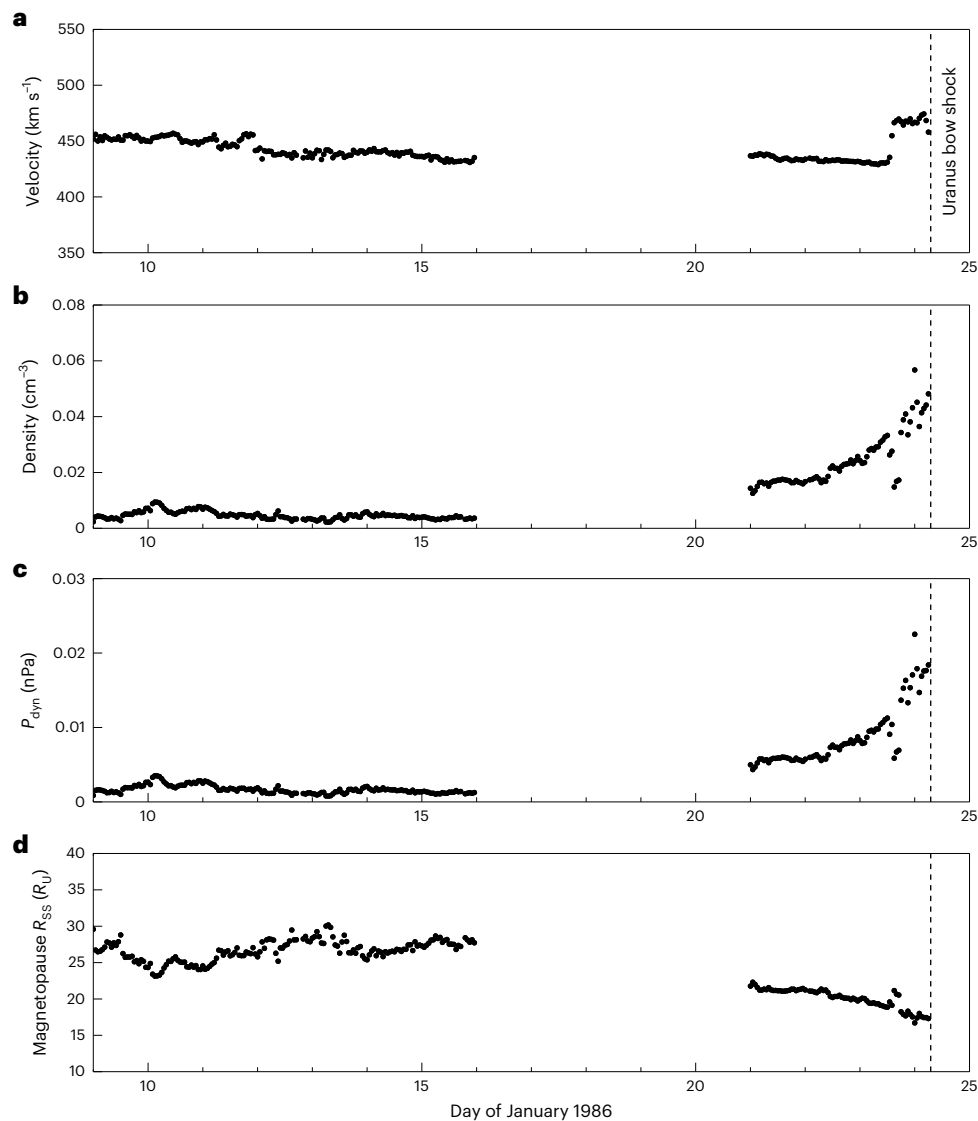
Fig. 1 | Voyager 2 in situ measurements of solar wind conditions upstream of Uranus, before the flyby. a–d , Measurements were made by the PLS. The dashed vertical line shows when Voyager 2 crossed Uranus’s bow shock on 24 January 1986 at 07:28 UT. The solar wind velocity ( a ), solar wind density ( b ), solar wind dynamic
