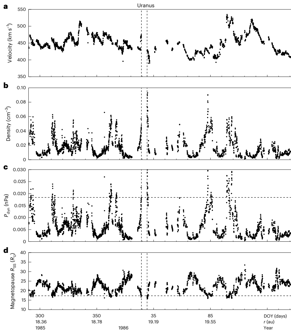
Fig. 2 | Voyager 2 in situ measurements of solar wind conditions at Uranus's orbit. a–d, Voyager 2 crossed Uranus's orbital path from day of year (DOY) 290 of 1985 until DOY 158 of 1986. This corresponds to Uranus's perihelion and aphelion heliocentric radial distances ( r ) of 18.28 au and 20.09 au, respectively. This figure is in the same format as Fig. 1. The solar wind velocity (a), solar wind density (b), solar wind dynamic pressure (c) and estimated expected magnetopause subsolar
