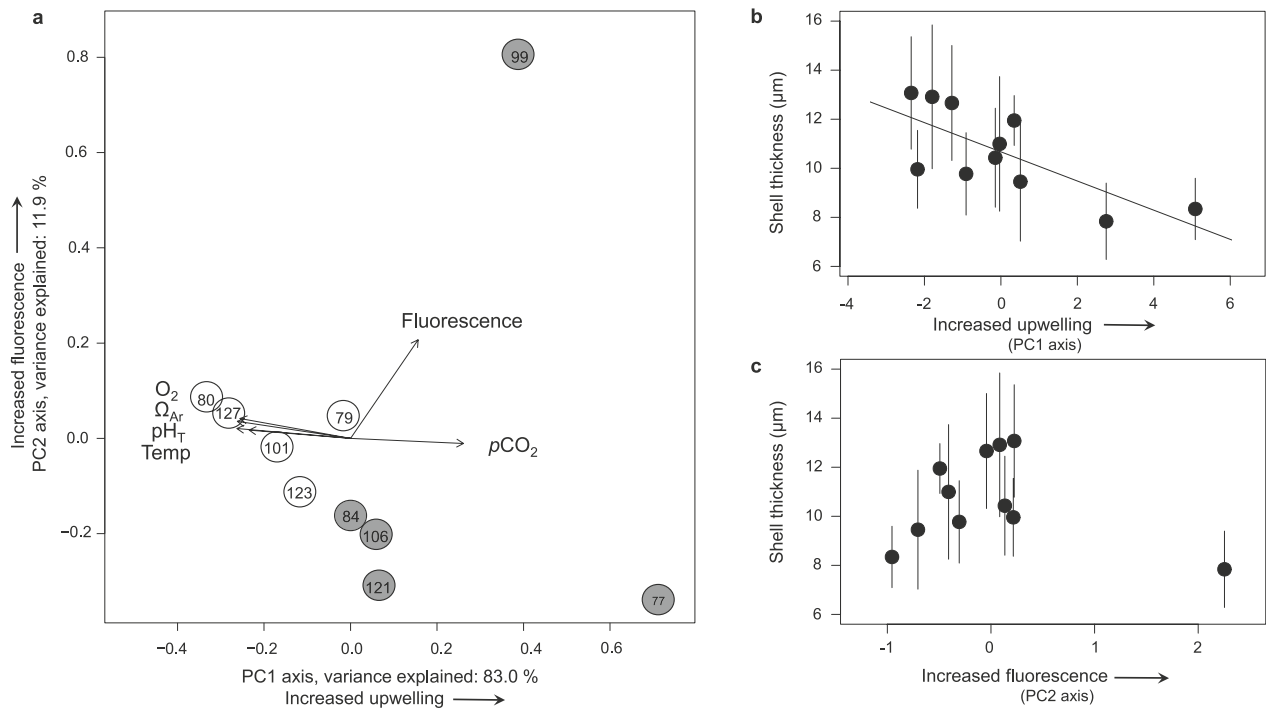
Figure 2. Relationships among ocean variables and average shell thickness of L. helicina pteropods. (a) Principal Component Analysis (PCA) based on aragonite saturation ( \Omega_{Ar} ), p\text{CO}_2 , pH, temperature (Temp), oxygen ( \text{O}_2 ) and chlorophyll fluorescence. The numbers within the plot represent the sampling stations used for analyses. Circles indicate stations with strong upwelling conditions nearshore (grey), and with less intense upwelling conditions offshore (white), see also Fig. 1. PC1 explains 83.0% of the variation among stations, and essentially reflects the offshore-onshore gradient driven by coastal upwelling. PC2 explains 11.9% of the variation, and is largely driven by variation in chlorophyll fluorescence. (b) Average shell thickness decreased significantly with PC1, associated with the upwelling gradient (principal component regression: y = -0.595 \text{ PC1} + 10.671 ; R^2 = 0.487 , N = 11 , p = 0.010 ). (c) Average shell thickness did not vary significantly with PC2, associated with chlorophyll fluorescence (principal component regression: R^2 = -0.058 , N = 11 , p = 0.519 ). Each dot in (b,c) represents the mean \pm SD of average shell thickness calculated over all 6–8 individuals per station. PC axes in the biplot (a) were scaled according to Gabriel (1971), whereas PC axes in (b,c) are unscaled.
