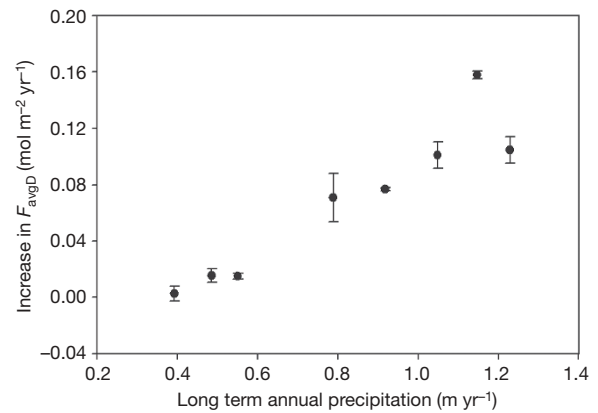
Figure 2 | Bin-averaged relationships between the increase in F_{\text{avgD}} and annual precipitation for sub-watersheds of the Mississippi. Non-responses from watersheds with low (<0.6 m yr -1 ) levels of precipitation are an indication of transport limitation. Only watersheds that had an increase in F_{\text{avgD}} were used. The error bars are \pm 1 s.e. ( n = 6 for each bin). The precipitation bins are 0.33–0.42 cm, 0.45–0.53 cm, 0.54–0.57 cm, 0.58–0.90 cm, 0.91–0.93 cm, 0.94–1.12 cm, 1.12–1.17 cm and 1.19–1.36 cm.
