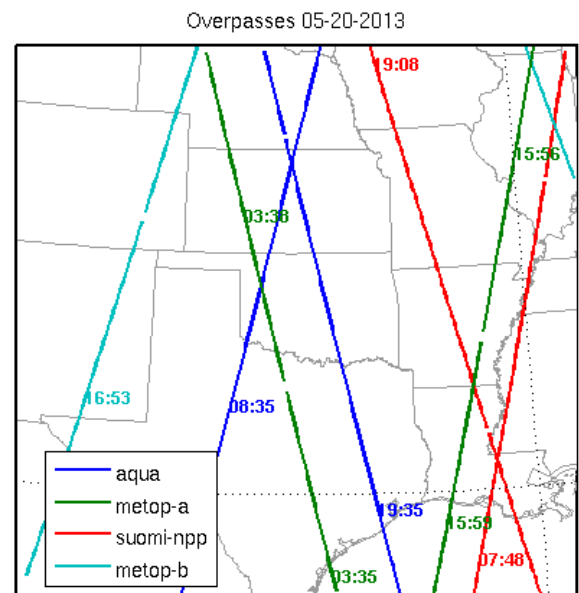
Figure 2: Satellite passes over Moore, Oklahoma
