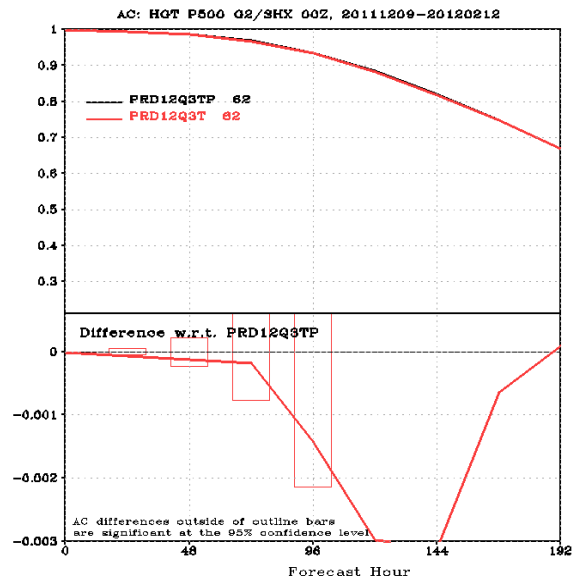
S. Hemisphere 500hPa Geopotential Height Anomaly Correlation
