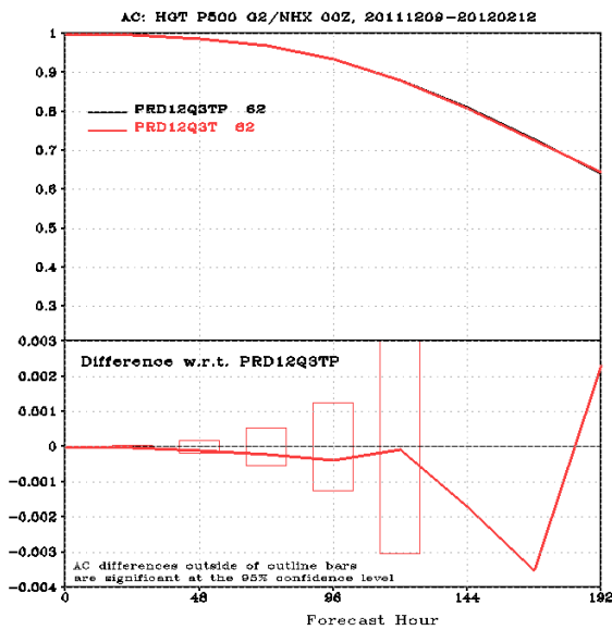
N. Hemisphere 500hPa Geopotential Height Anomaly Correlation
