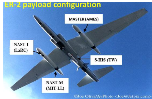
The NASA ER-2 research aircraft equipped with NAST-I, NAST-M, S-HIS and MASTER
