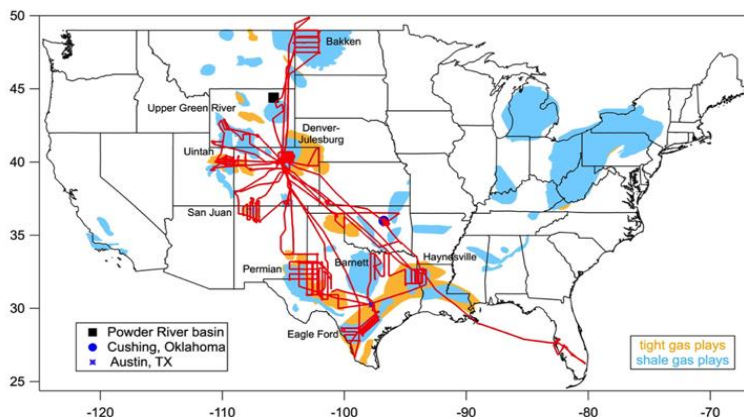
Flight tracks of NOAA's WP-3 aircraft during the 2015 SONGNEX campaign
