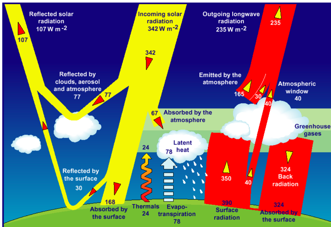
Climate System Energy Balance. Radiation Balance of the Earth (Jeffrey T. Kiehl and Kevin Trenberth) Image accessed from https://ceres.larc.nasa.gov/ceres_brochure.php?page=2
