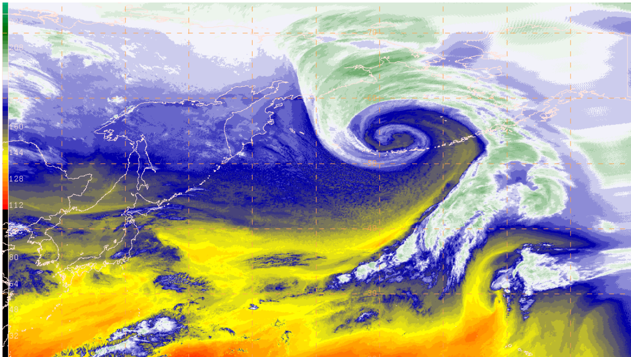
Hurricane-Force Low 0600 UTC on 12/13/15 using the 7.3 \mu m Low-Level Water Vapor channel on Himawari-8. Courtesy of JMA, NESDIS STAR, and CIRA.
