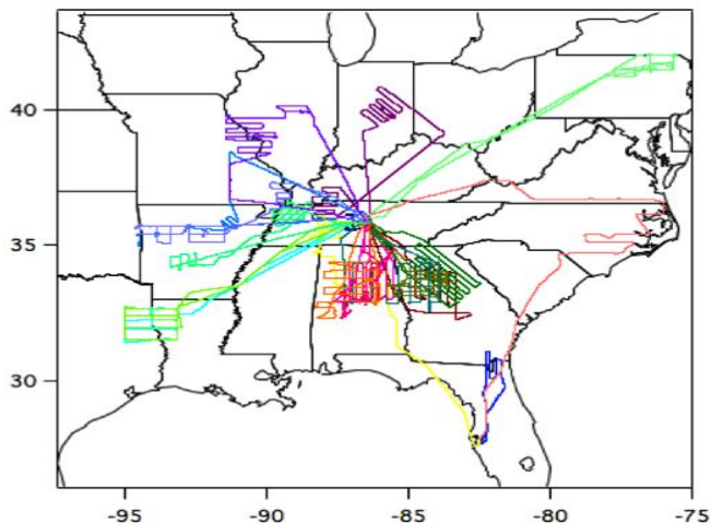
Flight tracks of NOAA's WP-3 aircraft during the 2013 SENEX campaign
