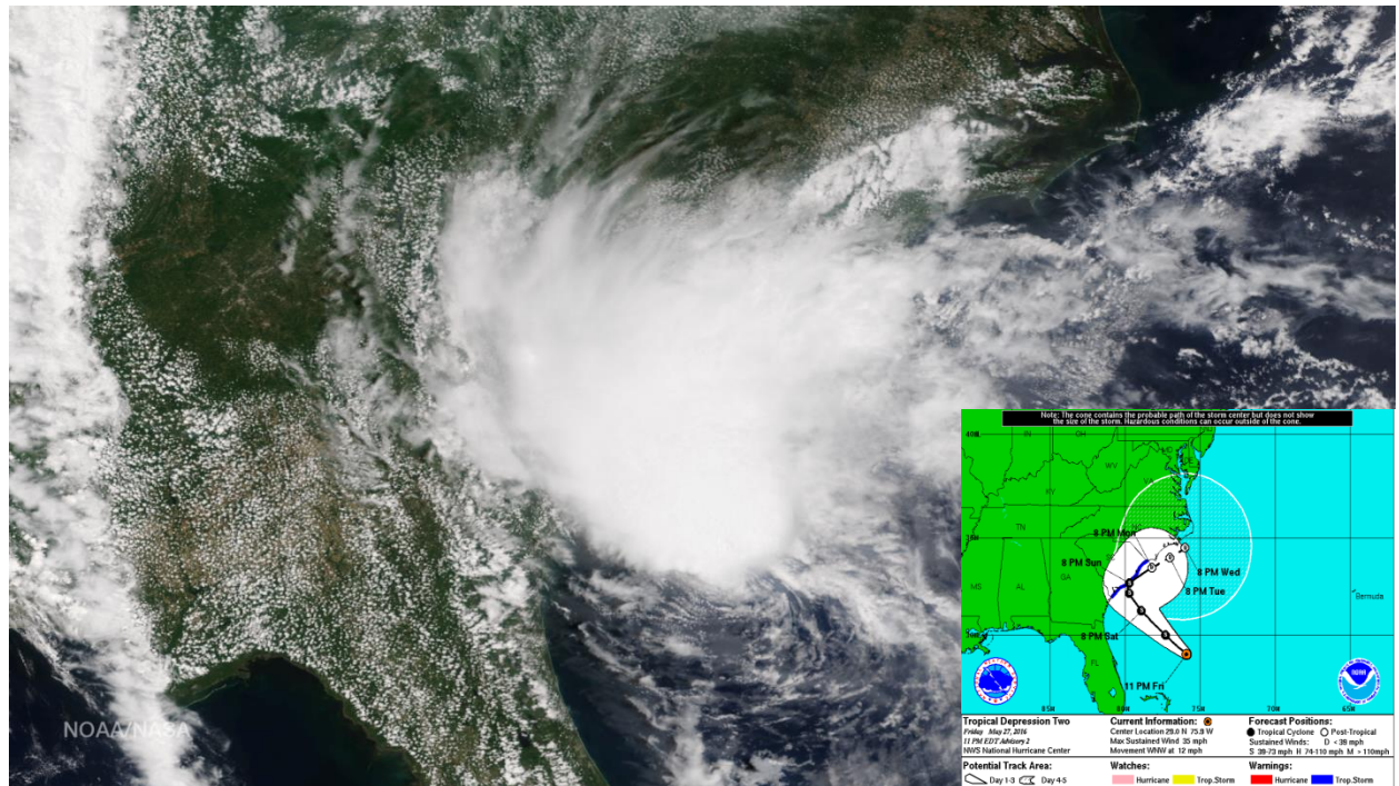
Tropical Storm Bonnie over the South Carolina Coast May 28, 2016. This image was taken by the Suomi NPP satellite's VIIRS instrument around 1910 UTC on May 28, 2016. Image courtesy NOAA Environmental Visualization Laboratory (NNVL) http://www.nnvl.noaa.gov/MediaDetail2.php?MediaID=1883&MediaTypeID=1 . Inset: National Hurricane Center 5-Day track forecast, uncertainty cone, and watch/warning, http://www.nhc.noaa.gov/archive/2016/graphics/al02/loop_5W.shtml
