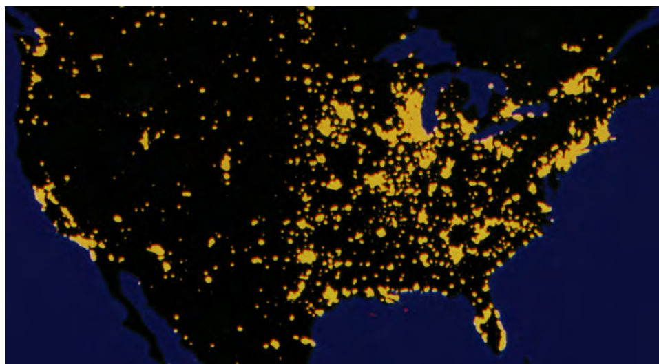
Sullivan, W.T. III, 1989, A 10 km resolution image of the entire night-time Earth based on cloud-free satellite photographs in the 400–1100 nm band. International Journal of Remote Sensing , v. 10, p. 1–5
