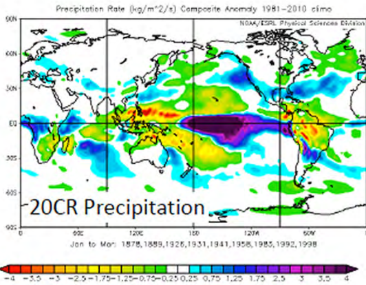
Maps from the NOAA-CIRES 20th Century Reanalysis version 2c (Compo et al. 2011, go.usa.gov/XTd ). ACRE, NOAA's NCEI, and 65 organizations are key partners providing historical observations to 20CR.
