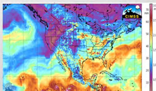
CIMSS MIMIC Total Precipitable Water 0000 UTC 21 July 2017
