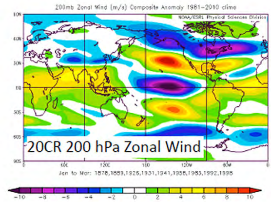
Maps from the NOAA-CIRES 20th Century Reanalysis version 2c (Compo et al. 2011, go.usa.gov/XTd ). ACRE, NOAA's NCEI, and 65 organizations are key partners providing historical observations to 20CR.
