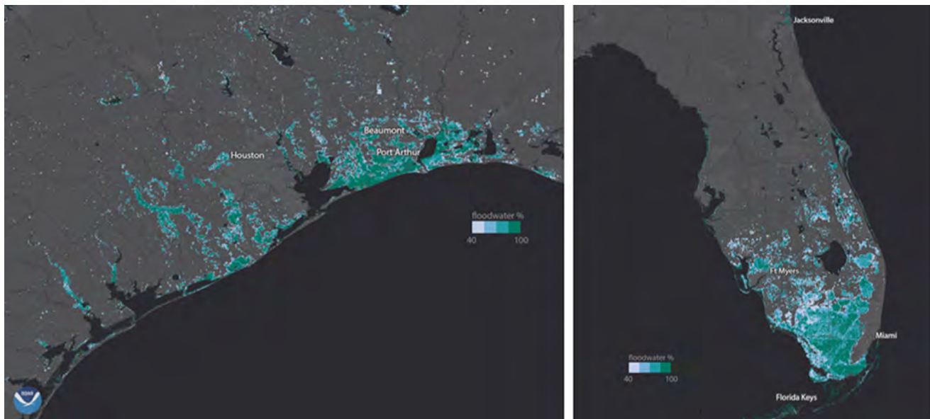
The turquoise color corresponds to areas of severe flooding.
