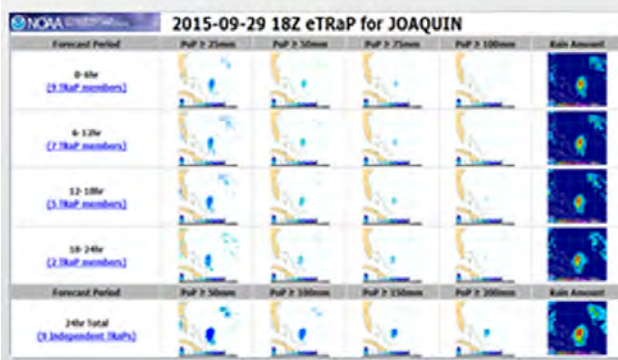
ensemble Tropical Rainfall Potential (eTRaP) 18 UTC 29 Sep 2015
