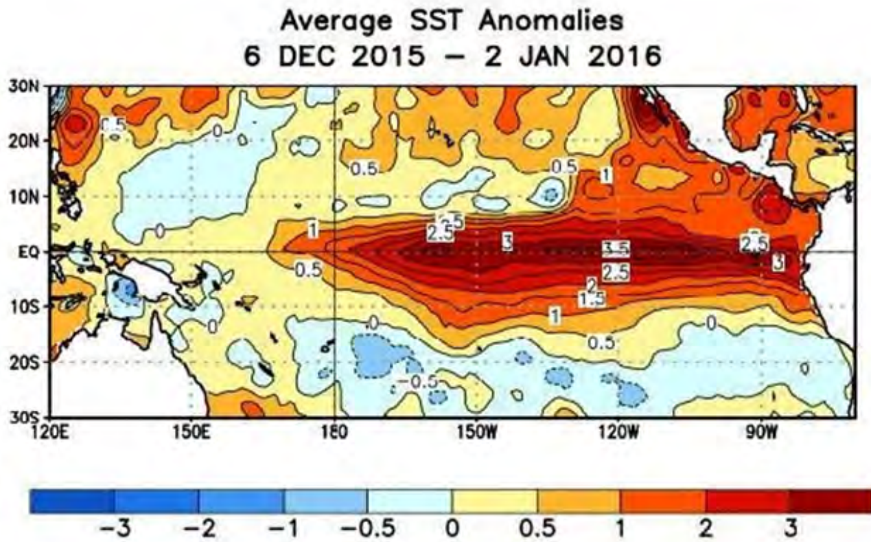
SST Departures (°C) in the Tropical Pacific during the last four weeks. NOAA, ENSO: Recent Evolution, Current Status and Predictions. Accessed from: https://www.ncdc.noaa.gov/monitoring-content/sotc/drought/2015/12/noaa-nws-cpc-160104-enso_evolution-status-fcsts-web.pdf
