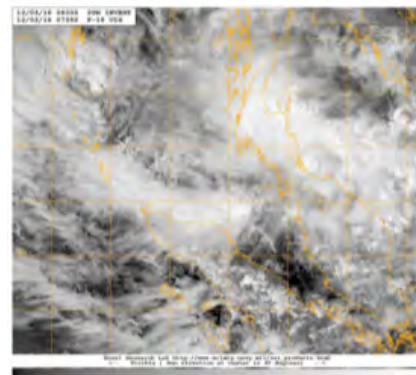
Images derived from VIIRS (top), AHI (middle), and the OLS (bottom) depicting a disturbance forming in the Strait of Malacca, located between the Malay Peninsula and the Indonesian island of Sumatra.
