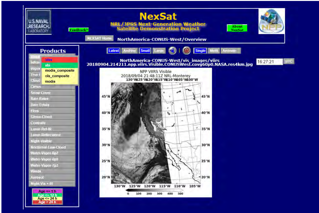
Screen shot of the product display showing visible imagery from VIIRS over the eastern Pacific and western U.S.
