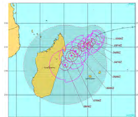
Automated Tropical Cyclone Forecasting System (ATCF) map that is tracking 09S.ENAWO as it approaches Madagascar.
