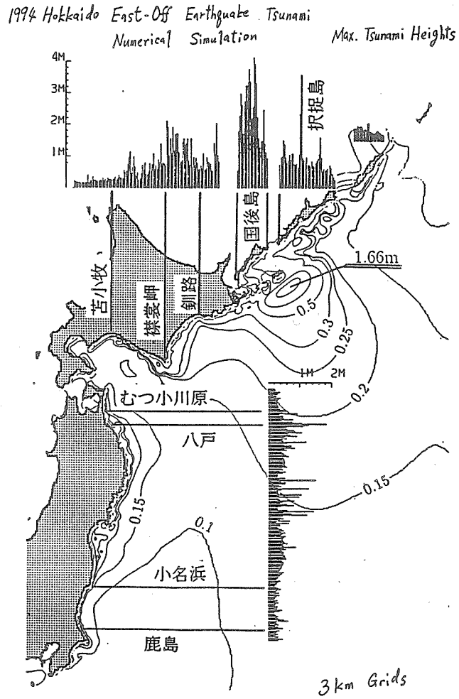
Fig. 9 Calculated Maximum Tsunami Heights along the Coasts
