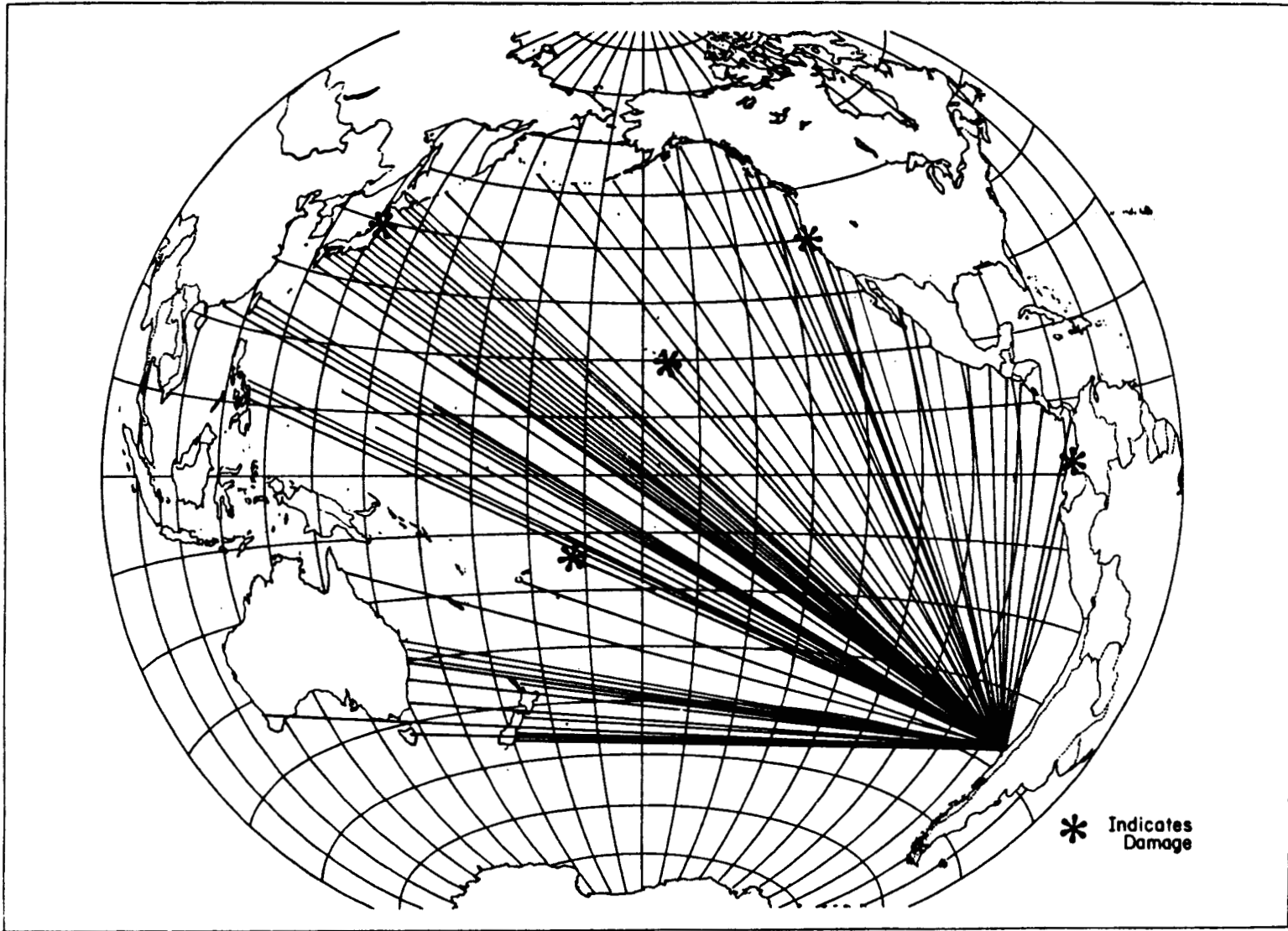
FIGURE 36. AREAS OUTSIDE PERU-CHILE REPORTING CHILE TSUNAMI OF MAY 22, 1960
